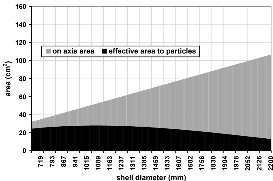
Fig. 8. The on axis geometric areas and effective areas to meteoroid particles predicted for the XEUS mirror shells.
