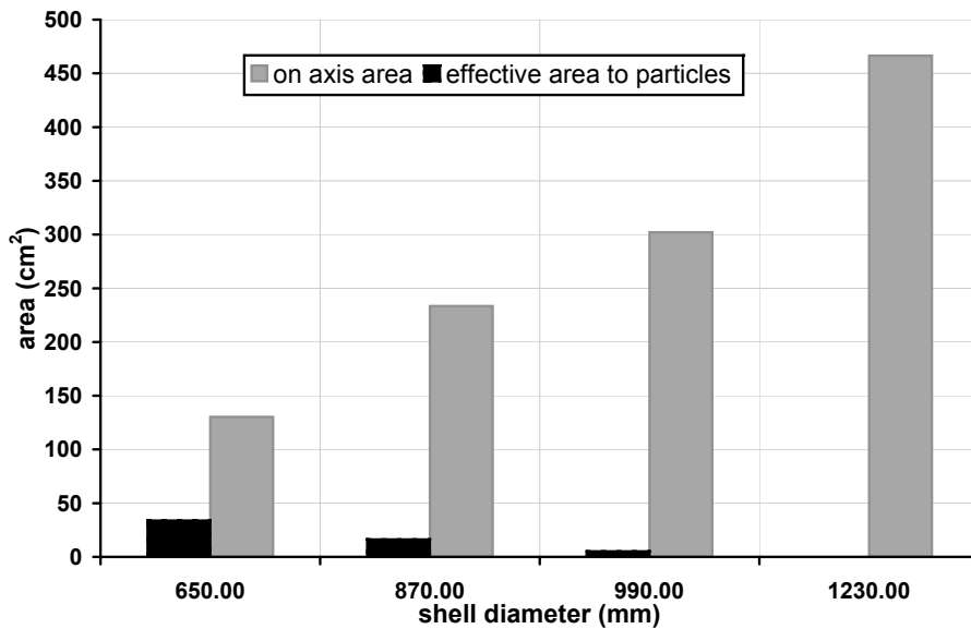
Fig. 4. The on axis geometric areas and effective areas to meteoroid particles of the Chandra mirror shells.
