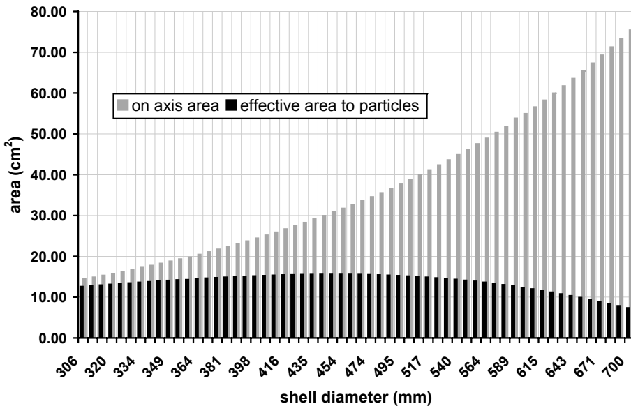
Fig. 3. The on axis geometric areas and effective areas to meteoroid particles of the XMM-Newton mirror shells.
