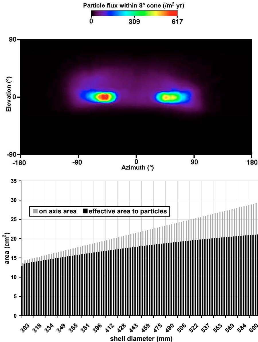
Fig. 6. The calculated flux of meteoroids and debris particles incident within 8^\circ of the Swift-XRT's optical axis as a function of pointing direction. The pointing direction of the telescope is measured in degrees from the the velocity vector of the spacecraft.
