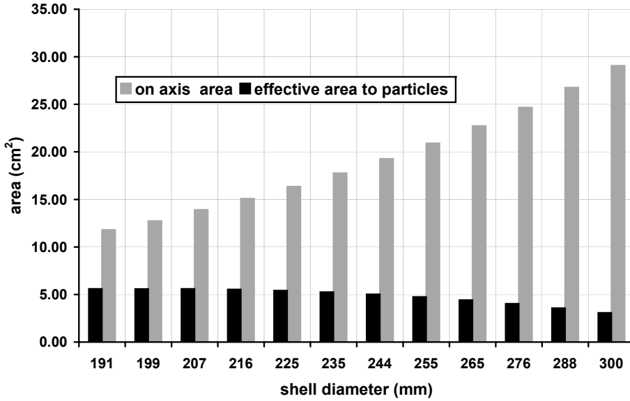
Fig. 2. The on axis geometric areas and effective areas to meteoroid particles of the Swift-XRT mirror shells.
