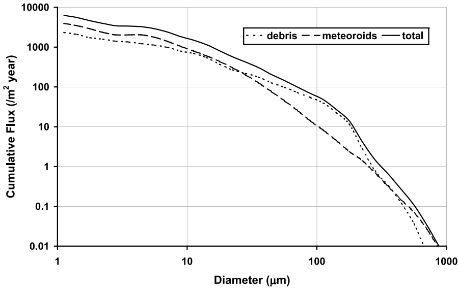
Fig. 5. The mean flux, as a function of particle diameter, of meteoroids and space debris particles incident on the Swift spacecraft calculated using the MASTER2005 model.
