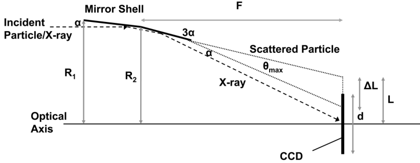
Fig. 1. The path of a focussed X-ray and the range of possible paths for a meteoroid particle after incidence on a Wolter type I mirror assembly in an X-ray telescope.
