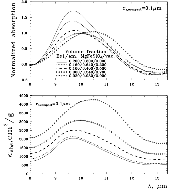
Fig. 2. Wavelength dependence of the normalised absorption efficiency factor ( upper panel ) and mass absorption coefficient ( lower panel ) for layered spheres with r_{\text{s}, \text{compact}} = 0.1\ \mu\text{m} . The particles consist of amorphous carbon (BeI), amorphous silicate with olivine composition ( \text{MgFeSiO}_4 ), and vacuum. The volume fraction of components V_i/V_{\text{total}} is indicated. The particles are of the same mass ( V_{\text{BeI}}/V_{\text{solid}} = V_{\text{BeI}}/(V_{\text{BeI}} + V_{\text{MgFeSiO}_4}) = 0.2 ), but of different porosity. The effect of variation of the silicate emission shape with the particle porosity is illustrated.
