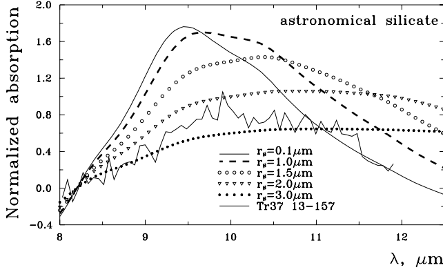
Fig. 1. Wavelength dependence of the normalised absorption efficiency factor [Q_{\text{abs}}(\lambda)/Q_{\text{abs}}(8.2\ \mu\text{m}) - 1] for compact spheres consisting of astronomical silicate. The effect of variation of the silicate emission shape with the particle size is illustrated. The observational profile of the T Tauri star Tr 37 13-157 (Sicilia-Aguilar et al. 2007) is shown for comparison. Note that this profile is not continuum subtracted.
