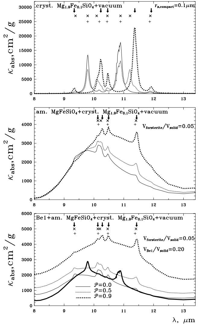
Fig. 5. Wavelength dependence of the mass absorption coefficient for compact and layered spheres with r_{\text{s,compact}} = 0.1\ \mu\text{m} . The particles consist of crystalline olivine and vacuum (upper panel), amorphous silicate, crystalline olivine, and vacuum (middle panel) and amorphous carbon, amorphous silicate, crystalline olivine, and vacuum (lower panel). The volume fraction of crystalline olivine and Be1 is indicated. The position of peaks is marked. The thick solid line at the lower panel shows the mass absorption coefficient for the mixture of compact grains (external mixing) with volume fractions of constituents corresponding to solid curve (internal mixing). The effect of variation of crystalline resonances with particle porosity and composition is illustrated.
