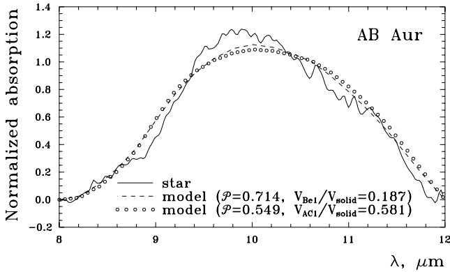
Fig. 4. The observational normalised profile of the 10\ \mu\text{m} feature for the Herbig Ae/Be star AB Aur (van Boekel et al. 2005; continuum is subtracted). The best fit profiles are shown for particles containing amorphous carbon in the form Be1 (dashed line) and AC1 (circles). The values of particle porosity \mathcal{P} and fractional amount of carbon V_{\text{Be1}}/V_{\text{solid}} are indicated.
