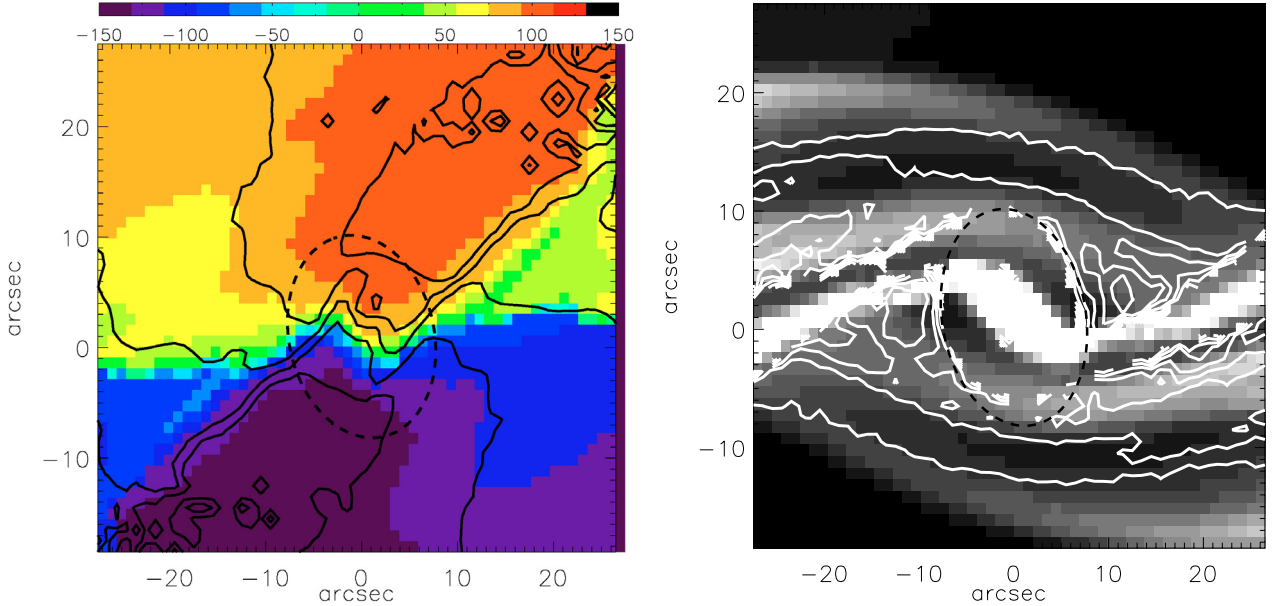
Fig. 1. In the left panel a ) the velocity field contours in the bar region, projected onto the plane of the sky, using i = 45^\circ and major axis of the galaxy at 57^\circ northwest (values from WSW01). Superposed are the isovelocity contours of the projected velocity field as derived in this work, with levels corresponding to intervals of 30 \text{ km s}^{-1} . In the right panel b ) density distribution from WSW01, superposed are the isodensity contours from the particle distribution of the SPH for the mass distribution of NGC 4123 derived from the I -band after 4 bar rotations. The non-axisymmetric component is fully grown after three bar rotations and the bar pattern speed is rotating clockwise in the inertial frame. Notice the agreement in the regions of high density within the bar region.
