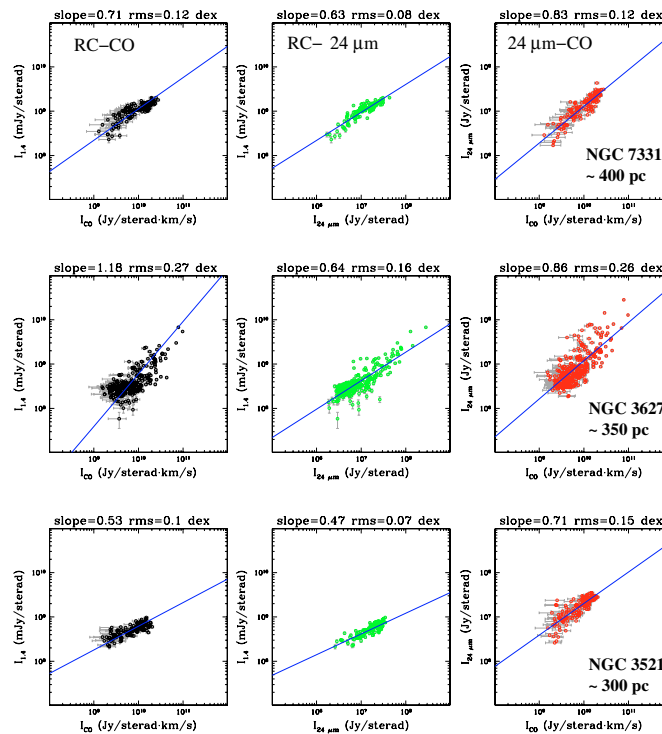
Fig. 1. RC-CO, RC-24 \mu\text{m} and 24 \mu\text{m} -CO correlations of NGC 7331, NGC 3627 and NGC 3521 at 6 arcsec resolution. The linear resolution achieved for each galaxy is indicated in the lower-right of the right-most panels.
