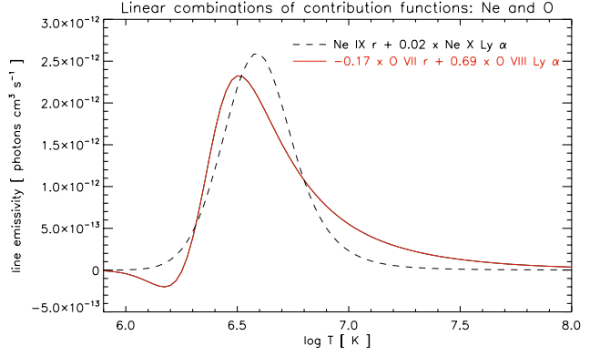
Fig. 3. Linear combinations of contribution functions of H-like Ly \alpha and He-like resonance lines of neon and oxygen.
