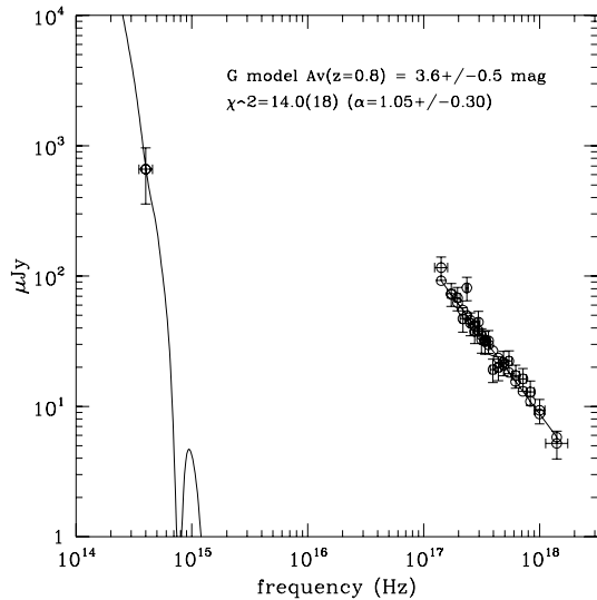
Fig. 3. The optical-to-X-ray afterglow spectrum from 95 s to 198 s after the burst. The X-ray data have been corrected for both the Galactic and the extra-galactic absorption. The optical data have been corrected only from the Galactic extinction. The solid line is the best-fit absorbed power-law model. We assumed a local extinction curve similar to the one observed in our Galaxy. The spectral index was fixed within the errors to the value derived only from the X-ray analysis.
