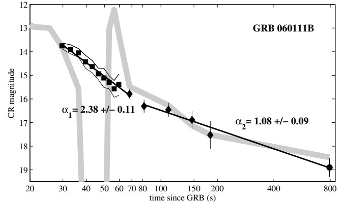
Fig. 2. light-curves of GRB 060111B. Black squares and diamonds with vertical error bars are CR magnitudes measured by TAROT (see Table 1). The black circle indicates the R magnitude measured by MITSuME (Yanagisawa et al. 2006). The solid straight lines are fits by a f(t) \propto t^{-\alpha} law. The broad grey line shows the high-energy light-curve ( -2.5 \log(\text{X-ray flux}) ) vertically offset to be compared to the optical light-curve. Before 75 s we extrapolated Swift-BAT flux to the 2–10 keV energy range. After 90 s, we used the XRT data in the 2–10 keV energy range (see Table 2).
