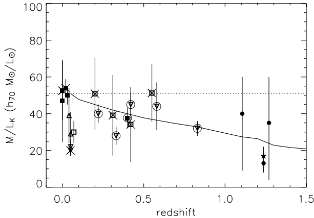
Fig. 9. The evolution of the restframe K band mass-to-light ratio. The filled circles are the M/L ratios from this work. The star shows the M/L determined for CI1252 using the T04 LF. The filled squares are K band M/L measurement from Rines et al. (2001), Kneib et al. (2003), Lin et al. (2003), Rines et al. (2004). The empty symbols show the K band M/L ratio derived from published M/L estimates in other passbands, i.e. B/B_j band (circle) from Girardi et al. (2000), Hoekstra et al. (2002), Sanderson & Ponman (2003), Gavazzi et al. (2004), R/r band (square) from Carlberg et al. (1997) and Andernach et al. (2004), and V band from Cirimele et al. (1997) and Hradecky et al. (2000) (see text). Crossed and circled points have masses determined from galaxy kinematics or strong/weak lensing respectively, at a difference with X-ray masses used in this work. The solid line traces the evolution expected from pure luminosity evolution of a simple stellar population formed at z = 5 , assuming that the cluster M/L ratio only evolves because of stellar evolution in galaxies, and neglecting any evolution in the dark mass. The dotted line shows the reference ( z = 0 ) value.
