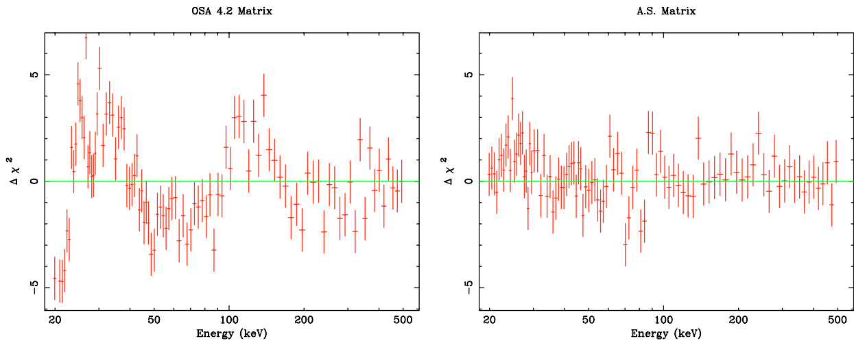
Fig. A.2. Left panel : residuals of the power law fit of the Crab spectrum obtained processing ISGRI data with the standard LUT2 and effective area. Right panel : residuals of the power law fit of the Crab spectrum obtained processing ISGRI data with the A.S. LUT2 and effective area.
