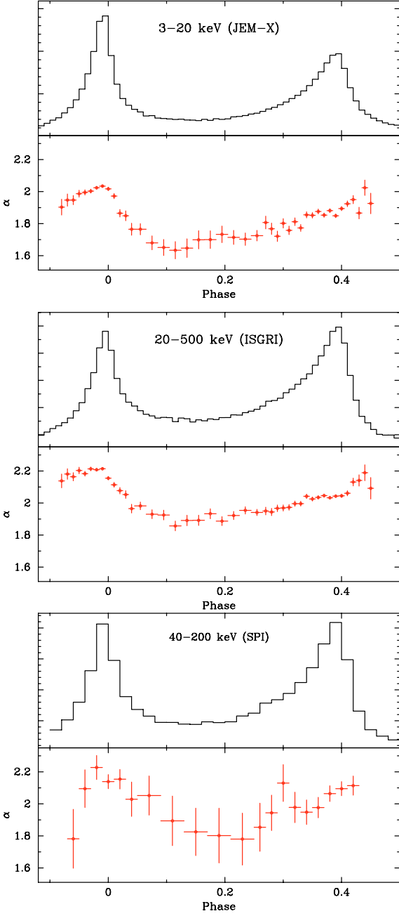
Fig. 2. Spectral index vs. phase measured by JEM-X in the energy range 3–20 keV ( top panel ), IBIS/ISGRI in the energy range 20–500 keV ( middle panel ) and SPI in the energy range 40–200 keV ( bottom panel ).
