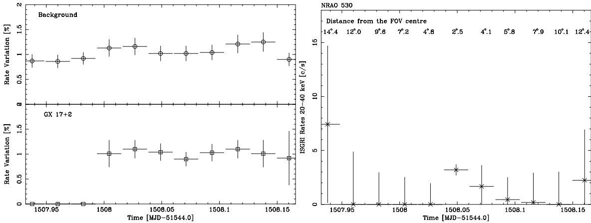
Fig. 2. Left, top: background rates normalized to the weighted average ( 79 \pm 12 c/s). Left, bottom: GX 17 + 2 rates normalized to the weighted average ( 10.9 \pm 0.9 c/s); in the first 3 ScW the source was outside the ISGRI FOV. Right: NRAO 530 rates; upper limits are at 3\sigma . In the top of the figure, the distance of the source from the ISGRI FOV centre is shown in every ScW. All the lightcurves are in the 20–40 keV energy band.
