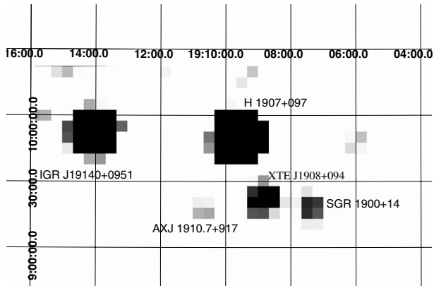
Fig. 1. IBIS/ISGRI image of the SGR 1900+14 field in the 18–60 keV energy range. The other detected sources are the high-mass X-ray binary (HMXB) IGR J19140+0951 (Rodriguez et al. 2005), the black hole candidate XTE J1908+094 (in’t Zand et al. 2002), the HMXB pulsar H 1907+097 (Makishima et al. 1984), and the weak unidentified source AXJ 1910.7+917 (Sugizaki et al. 2001).
