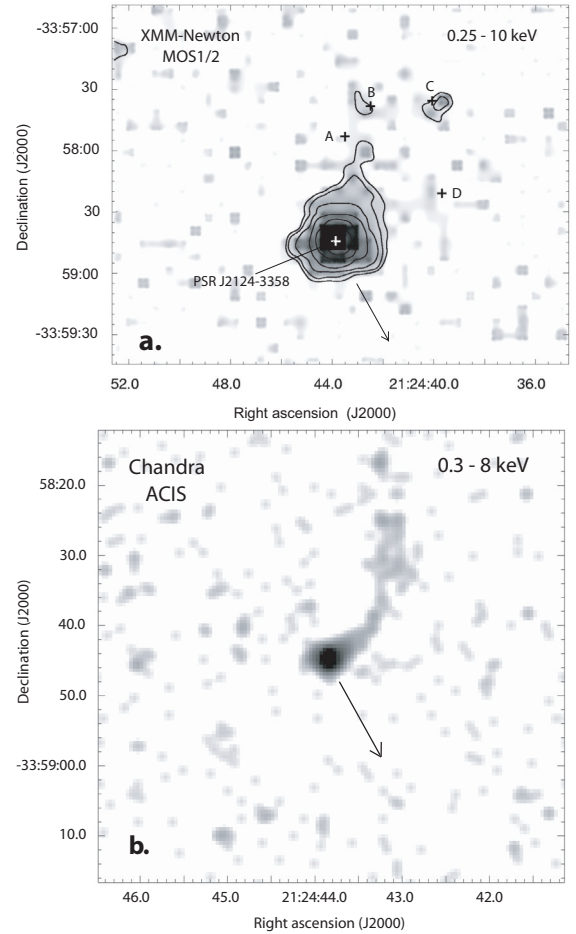
Fig. 1. a) XMM-Newton MOS1/2 image of PSR J2124–3358 with overlaid contours. The pulsar proper motion is indicated by an arrow. The position of bright stars located in the 1.5 arcmin neighborhood of PSR J2124–3358 are indicated. b) PSR J2124–3358 as seen by the ACIS detector aboard Chandra.
