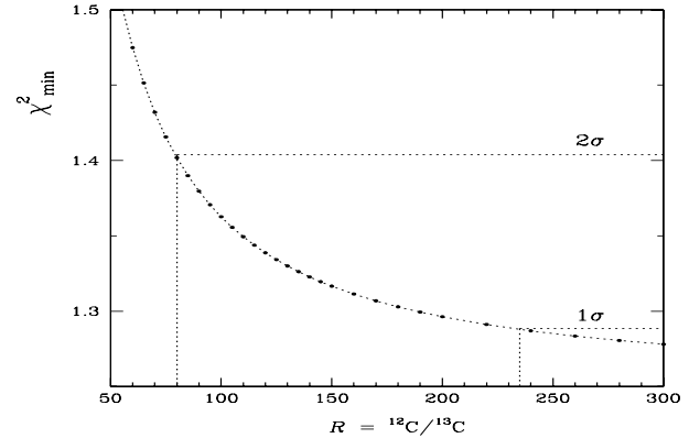
Fig. 2. Confidence intervals in the “ \chi^2 - \mathcal{R} ” plane calculated from the simultaneous fit of the \text{CI}^* lines shown in Fig. 1.
