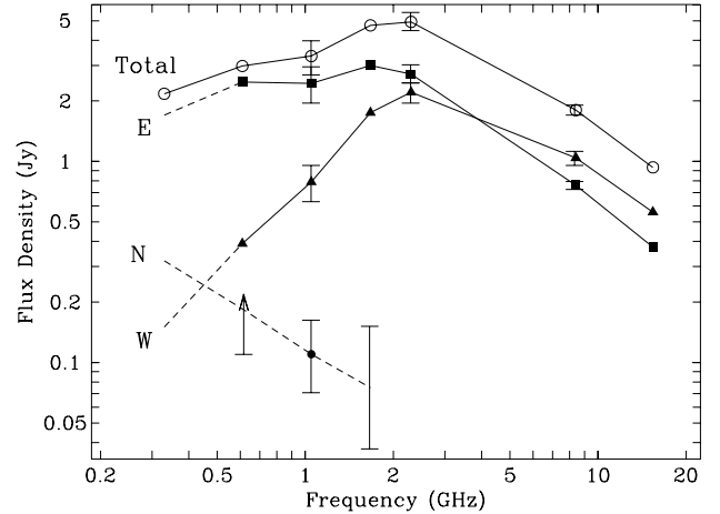
Fig. 7. Continuum component flux densities at multiple frequencies, based on data at 0.33, 0.61, 1.67, 2.3, and 8.4 GHz from LF, at 2.3, 8.4, and 15.4 GHz from K03, and at 1.049 GHz from our own observations. See Sect. 4 for details.
