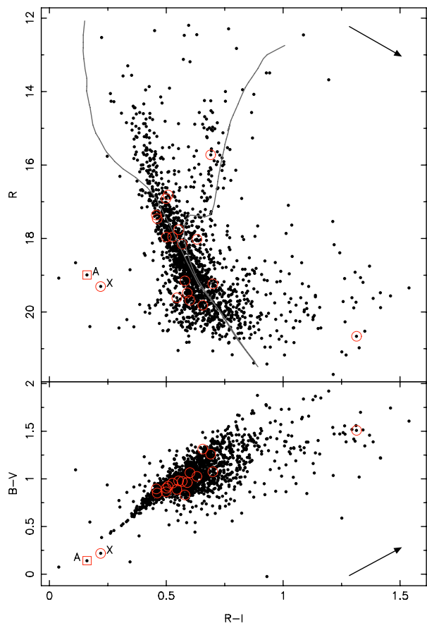
Fig. 2. Top : a colour-magnitude and colour-colour diagram ( bottom ) of the BVRI photometry of the 1A 1246–588 region. Stars inside the ROSAT error circle (Fig. 1) are encircled. Also shown in the CMD are two solar metallicity isochrones from Girardi et al. (2000), placed at a distance of 4.0 kpc and an absorption of A_V = 1.0 . The left is for an age of 0.1 Gyr, while the right has an age of 10 Gyr. These isochrones are merely to guide the eye, as there will be a spread in distance, age, metallicity and absorption. The arrows indicate the effects of absorption, where the length of the arrow is for an extra absorption of \Delta A_V = 1.0 . Of the stars present in the error circle, star X is exceptionally blue and the likely optical counterpart to 1A 1246–588. Star A has similar colours and magnitudes as star X, but is located outside the 95% confidence error circle.
