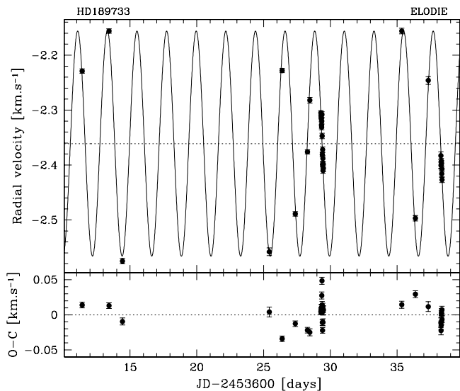
Fig. 1. Radial-velocity measurements of HD 189733 superimposed on the best Keplerian solution. The higher density of points corresponds to spectroscopic-transit measurements. They are not used to derive the Keplerian solution. Error bars represent the photon-noise uncertainties.
