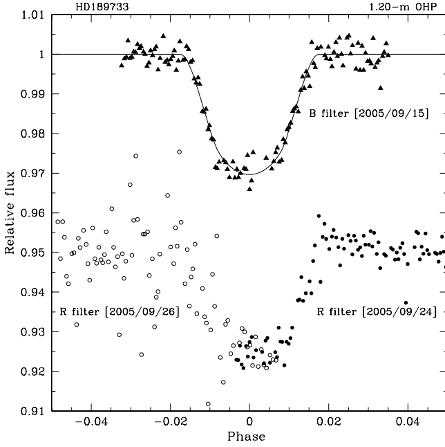
Fig. 3. Photometric transits of HD 189733 observed with the 1.20-m OHP telescope. Triangles correspond to the observation on B band made on September 15th 2005. Full circles and open circles correspond to observation on R band made respectively on September 24th and 26th 2005. The solid curve represents the best-fit model for the complete B -band transit.
