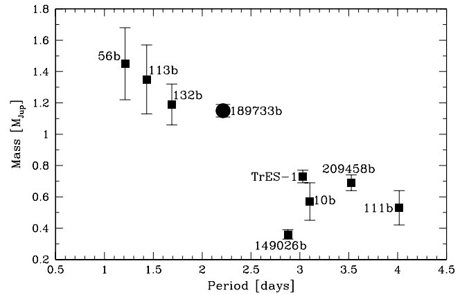
Fig. 5. Mass-period diagram for the 9 transiting exoplanets.
