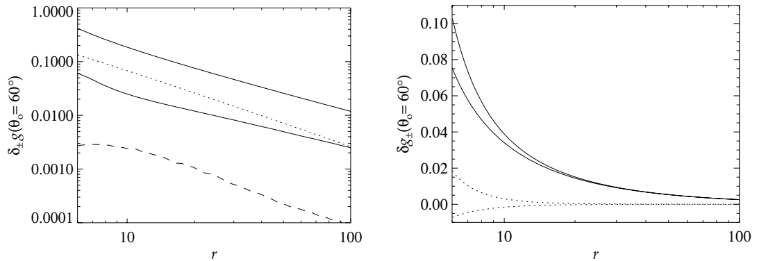
Fig. 2. Left: the dependence of the maximum and minimum relative error \delta_{\pm}g(r, \theta_o) of g -factor on the radius for inclination angle \theta_o = 60^\circ , in logarithmic scale. Solid lines are for the approximation (12) (upper for the maximum, lower for the minimum), dotted line is for the approximation (14) and dashed line is for the approximation (17). Right: the relative error \delta g_{\pm}(r, \theta_o) of the extremal values of g -factor. The solid lines are for Eq. (13) and the dashed lines are for Eq. (15). Upper lines show the relative error of g_+ , lower lines are for the relative error of g_- . The relative error for the approximation (2) is better than 0.1% and thus it is not plotted here.
