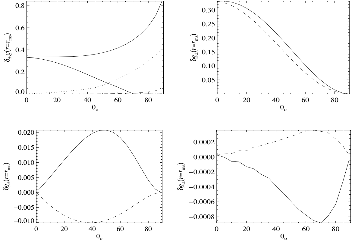
Fig. 1. Accuracy assessment for different approximation formulae. (i) Top row – left panel: the dependence of the maximum and minimum relative error \delta_{\pm}g(r, \theta_o) of the g -factor on observer's inclination angle \theta_o for a narrow ring, r = r_{\text{ms}} . Solid lines refer to Eq. (12) (the upper one is for maximum, the lower one is for minimum); the dotted line refers to Eq. (14); the dashed line is for Eq. (17). The approximation formula (12) is the worst of the three cases in the sense that it has a significant non-zero value of the minimum error. This is due to neglecting aberration. The relative error \delta g = |g_{\text{approx}} - g|/g is determined with respect to exact (numerically computed) values. (ii) Top row – right panel: the relative error \delta g_{\pm}(r, \theta_o) of the extremal values of g -factor for a ring r = r_{\text{ms}} as a function of observer's inclination angle. The relative error \delta g_{\pm} = (g_{\text{approx}}^{\pm} - g_{\pm})/g_{\pm} of the extremal values is again determined with respect to exact values from equation of geodesic. The solid/dashed lines are for maximum/minimum of g -factor; both lines are for the approximation (13). (iii) Bottom row – left panel: the same as top right but with the approximation (15). (iv) Bottom row – right panel: the same as top right but for the approximation (2).
