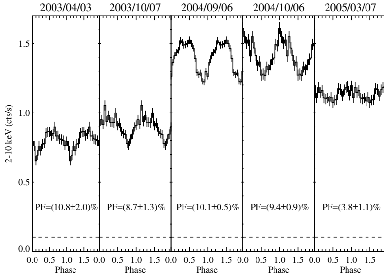
Fig. 1. Background subtracted pulse profiles in the 2–10 keV energy range of SGR 1806–20 as seen by the PN camera during the five XMM-Newton observations (the dates of the observations are reported at the top of each panel). The dashed line shows the blackbody contribution to the phase averaged count rate when the source spectrum is fitted using an absorbed power-law plus blackbody, with the absorption and blackbody parameters linked to the same value during the five observations (last line in Table 1). The pulsed fractions (PF) computed from a sinusoidal fit of the profiles are also indicated.
