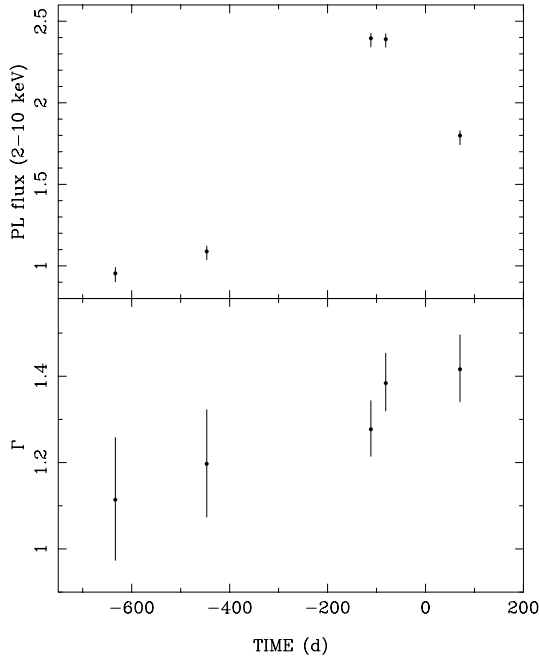
Fig. 2. Flux of the power-law component (in units of 10^{-11} erg \text{cm}^{-2} \text{s}^{-1} ) and power-law photon index during the five XMM-Newton observations. The source spectra are fit simultaneously using an absorbed power-law plus blackbody with only the power-law parameters free to vary independently during the five observations. The origin of the time axis corresponds to the giant flare of 2004 December 27.
