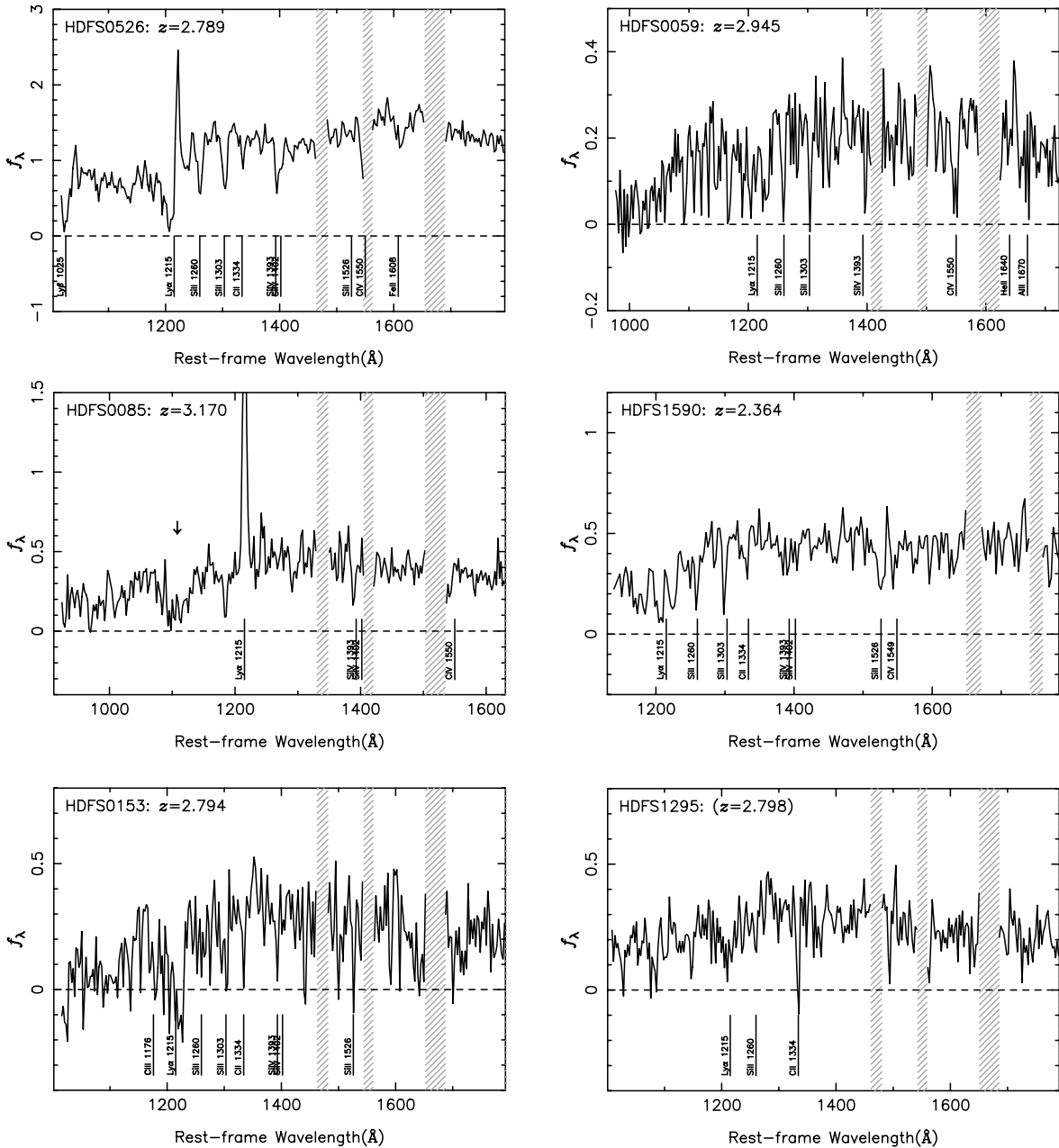
Fig. 2. The rest-frame UV spectra of galaxies with redshift identifications. Objects are shown as an order of I_{814} magnitude. The spectra were 3-pixel binned. Units of f_{\lambda} is 10^{-16} erg/s/cm ^2 /Å. The hatched areas represent the wavelength ranges dominated by atmospheric lines and where we do not show objects' spectra. The redshifts with parentheses indicate that the redshift determination is not definitive. An arrow in the panel of HDFS0085 indicates a position of Ly \alpha line at z = 2.8 , which coincides with a trough in the continuum (see Sect. 3.2).
