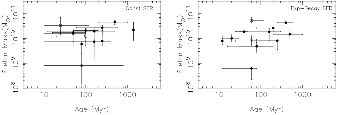
Fig. 7. Ages and stellar mass estimates for star-forming galaxies in the HDF-S. The meanings of symbols and error bars are the same as Fig. 6.
