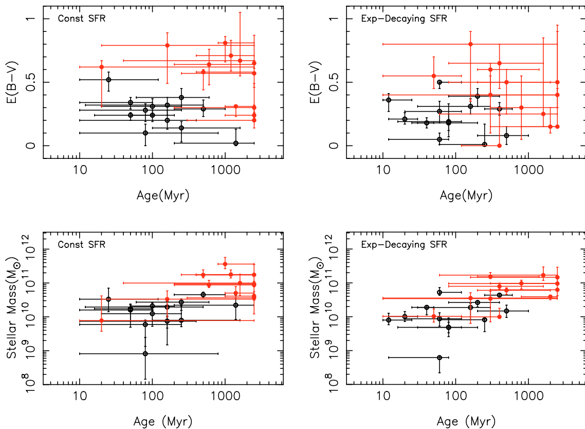
Fig. 8. Distribution of ages, dust attenuation and stellar mass estimates obtained as a result of SED fitting for star-forming galaxies (open circles) and distant red galaxies (red filled circles) in the HDF-S. In the left two panels, the models assume the constant SFH and in the right panels the models with exponentially-decaying SFH were used for comparison with observed SEDs. All calculations of stellar populations in models in these diagrams were started from metal-free gas. The error bars indicate the ranges covered by 68% confidence levels.
