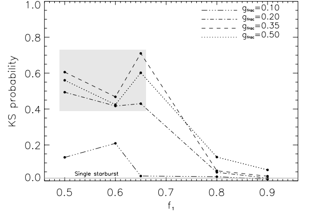
Fig. 3. Best KS probabilities for various values of f_1 and for four final gas fractions g_{\text{frac}} . The shaded region shows a set of degenerate models that have high KS probabilities and therefore cannot be discounted completely. The KS probability for a single starburst scenario is shown by the solid line at 2 percent.
