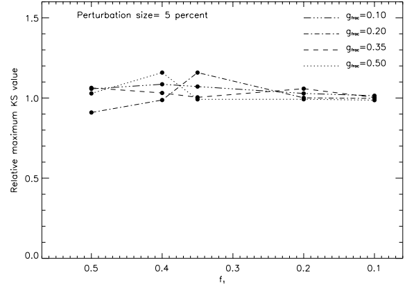
Fig. 7. KS values for perturbed double starburst scenarios as a fraction of the KS values in the unperturbed case. The size of the perturbation applied to the system is 5 percent.
