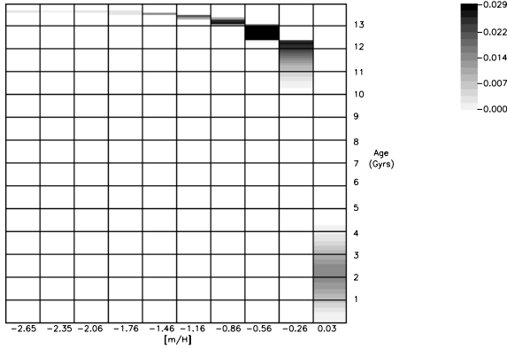
Fig. 5. Age-metallicity grid showing the fraction of stellar mass predicted by the favoured model as a function of age and metallicity. The key indicates stellar fractions corresponding to the levels of shading in the plot.
