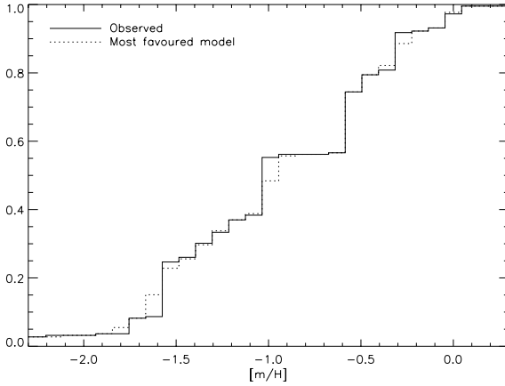
Fig. 6. Comparison between observed MDF and that predicted by the favoured model (which gives the highest KS probability).
