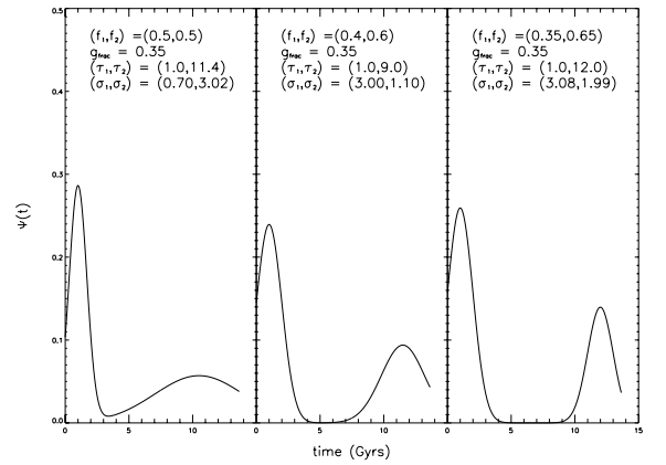
Fig. 4. Three GC formation histories corresponding to the best KS probabilities shown in the shaded region in Fig. 3.
