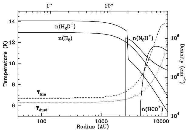
Fig. 3. Radial profiles of dust and gas temperature, and the densities of \text{H}_2 , \text{H}_2\text{D}^+ ( \times 2 \times 10^9 ), \text{HCO}^+ ( \times 10^{12} ) and \text{N}_2\text{H}^+ ( \times 10^{10} ) in our model of LDN 1544.
