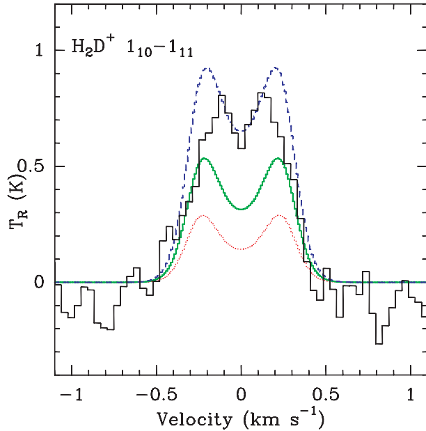
Fig. 10. Results of models with the temperature density distributions from Young et al., a “jump” in b_D at R = 10^3 AU, and with the \text{H}_2\text{D}^+ collisional rate coefficient at the standard value and increased by factors of 3 and 10 (curves from bottom to top), superposed on the observations (histogram).
