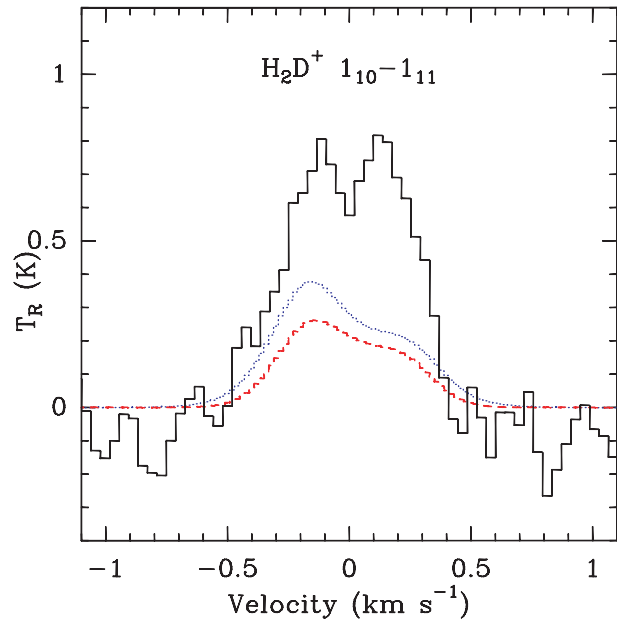
Fig. 9. Results of models with a power-law density distribution, T_{\text{kin}} \equiv 10 \text{ K} , Hunter’s velocity profile “11d”, and with the \text{H}_2\text{D}^+ abundance constant (dotted line) and with an inner hole (dashed line), superposed on the observations (histogram).
