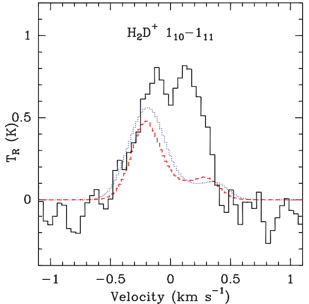
Fig. 8. Results of models with a power-law density distribution and the gas temperature calculated by Young et al., the effect of depletion included for a chemical age of 0.1 Myr for either a constant infall velocity (dotted line) or the Ciolek & Basu velocity field (dashed line), superposed on the observations (histogram).
