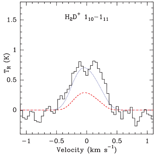
Fig. 4. Results of 2D models with T_{\text{kin}} \equiv 10 K (dotted line) and with the temperature distribution from Galli et al. (dashed line), superposed on the observations (histogram).
