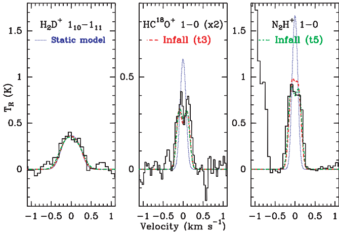
Fig. 2. As Fig. 1, at 20 arcsec offset (average NSEW).
