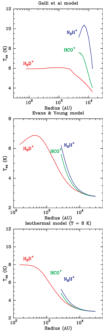
Fig. 5. Excitation temperature profiles of \text{H}_2\text{D}^+ 1_{10-111} for the physical structures by Galli et al. ( top ), Young et al. ( middle ), and for the isothermal power-law model ( bottom ). Within the radius of high \text{H}_2\text{D}^+ abundance ( \sim 3000 AU), T_{\text{ex}} is practically constant in the Galli case, but has a gradient in the other cases.
