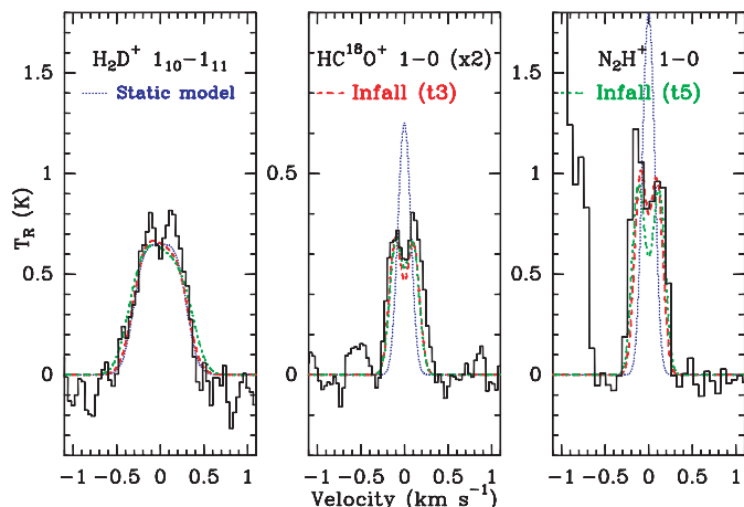
Fig. 1. Line profiles of \text{H}_2\text{D}^+ (left), \text{HC}^{18}\text{O}^+ (middle) and \text{N}_2\text{H}^+ (right; only the F_1F = 1,0\text{--}1,1 hyperfine component) observed towards the “dust peak” of LDN 1544. Superposed are synthetic profiles for the best-fit static model (dotted), and infall models after Ciolek & Basu (2000) for times 2.660 (dashed) and 2.684 Myr (dash-dotted). The line width (static: b_D = 0.15 \text{ km s}^{-1} ; infall: b_D = 0.05 \text{ km s}^{-1} ) is set to match the \text{H}_2\text{D}^+ data.
