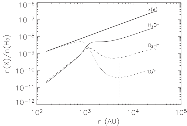
Fig. 7. Calculated abundances of \text{H}_2\text{D}^+ , \text{D}_2\text{H}^+ and \text{D}_3^+ for an age of 0.1 Myr, a cosmic-ray ionization rate of 3 \times 10^{-17} \text{ s}^{-1} and the physical structure by Evans et al. (2001). The dotted lines indicate the radii equivalent to one and two CSO beams, for comparison with observations.
