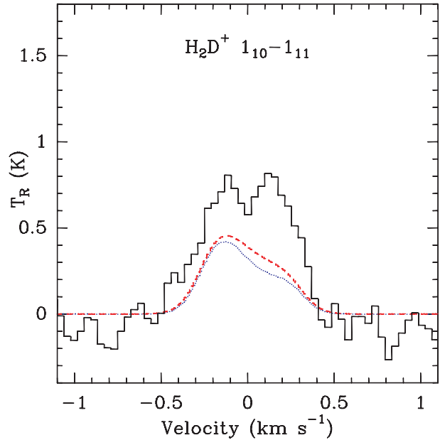
Fig. 6. Results of models with a power-law density distribution and T_{\text{kin}} \equiv 8 K (dotted line) and with the gas temperature calculated by Young et al. (dashed line), superposed on the observations (histogram).
