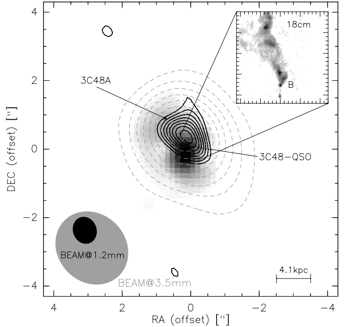
Fig. 2. Contours of the 3.5 mm ( grey dashed lines ) and 1.2 mm ( black solid lines ) continuum observed in 2003. The contours are the same as in Fig. 1, and are superposed on the greyscale NIR-image (Zuther et al. 2004) with the QSO nucleus subtracted (its position agrees with the radio QSO position and is thus located at zero in our maps). The radio jet at 18 cm is plotted in the small box ( upper right ; from Wilkinson et al. 1991; tickmarks correspond to 0.1'' ). B denotes the position of the QSO.
