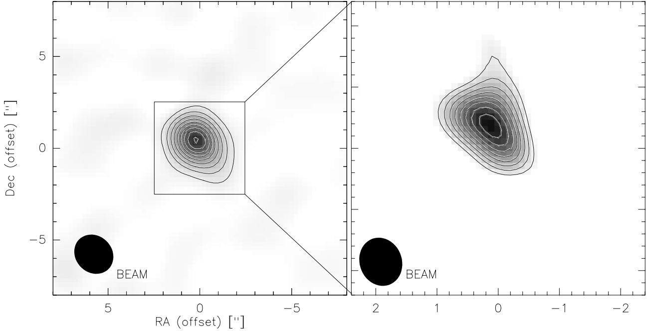
Fig. 1. Continuum maps at 3.5 mm ( left ) and 1.2 mm ( right ) made with the IRAM interferometer in 2003, shown as both contours and greyscale. Contour levels at 3.5 mm are 0.025 to 0.23 by 0.025 Jy/beam ( 20\sigma ). Contour levels at 1.2 mm are 0.01 Jy/beam ( 5\sigma ) to 0.044 Jy/beam by 0.004 Jy/beam ( 2\sigma ). Both maps were made with uniform weighting. Beams are 2.3'' \times 2.0'' at PA = 44^\circ at 3.5 mm and 0.8'' \times 0.7'' at PA = 20^\circ at 1.2 mm.
