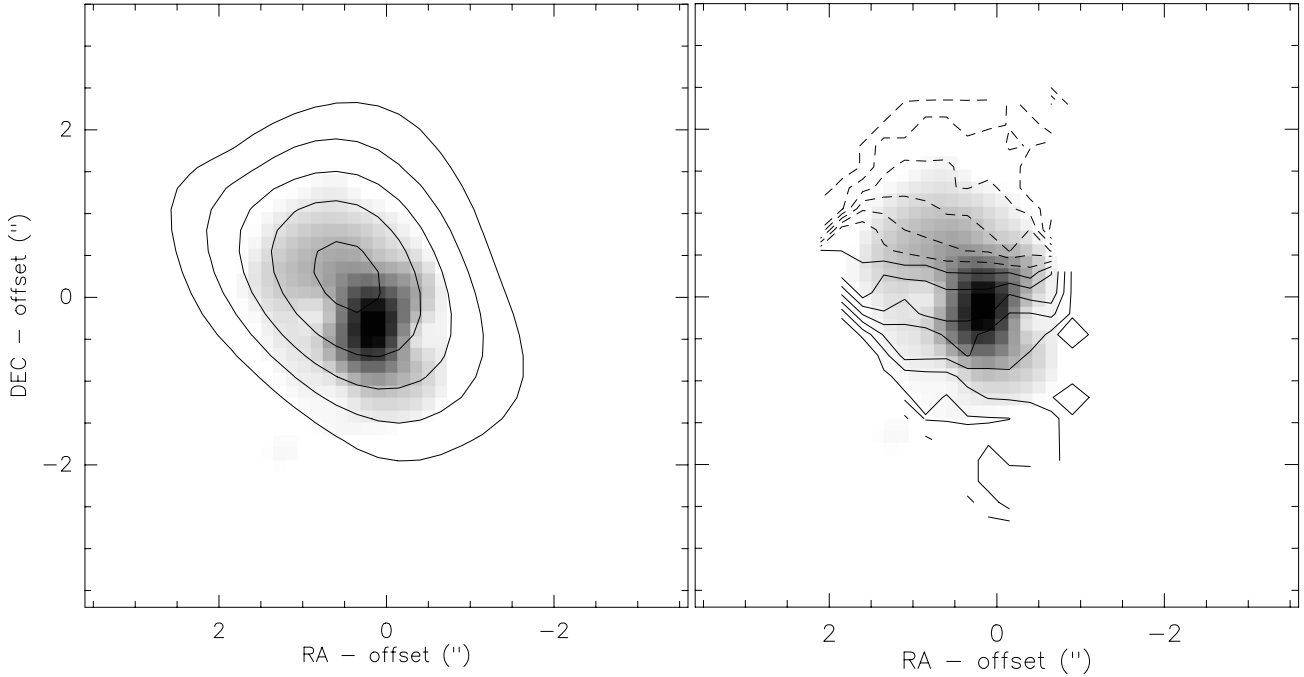
Fig. 11. Left: 3C 48 integrated CO(1–0) emission from -120 to +80 \text{km s}^{-1} . Contours are 0.2 to 0.8 \text{Jy beam}^{-1} \text{ km s}^{-1} by 0.1 \text{Jy beam}^{-1} \text{ km s}^{-1} . The CO beam is 3.5'' \times 2.6'' . Right: CO isovelocity map. Velocity contours run from -95 to -45 \text{km s}^{-1} ( dashed ) and -35 to 25 \text{km s}^{-1} ( solid ) in steps of 10 \text{km s}^{-1} . Both CO maps are superposed on the NIR image of Zuther et al. (2004) ( grey scale ). Data are taken from the merged 1995 and 2003 data sets.
