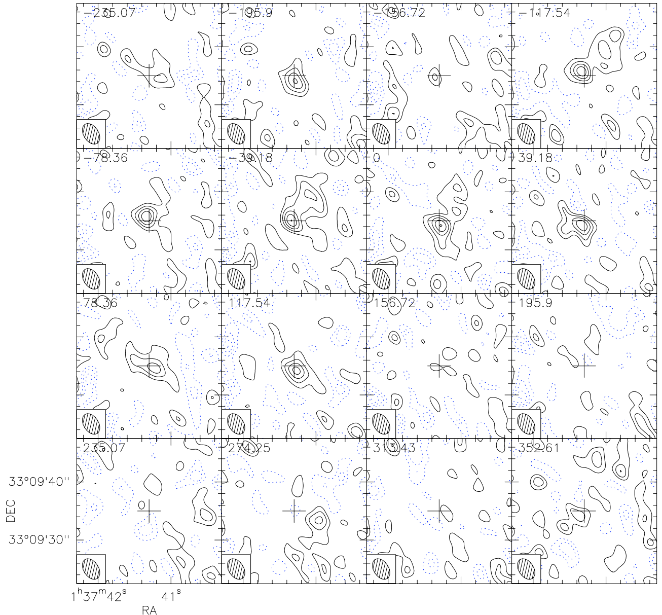
Fig. 6. CO(1–0) channel maps from the merged 1995+2003 data. Positive and negative contours are in steps of 1.2 \text{ mJy beam}^{-1} ( 1\sigma ), up to a maximum of 6.0 \text{ mJy beam}^{-1} . The natural weighted beam is 3.6'' \times 2.5'' at \text{PA} = 32^\circ . The cross in the maps denotes the phase center (Sect. 2).
