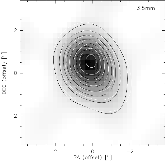
Fig. 5. Continuum emission at 3.5 mm (grey scale and black solid contours; 2003 data only) overlaid with contours of a three Gaussian component model taken from 1mm with corrected fluxes and smoothed to the 3.5 mm beam (white solid lines). Contours of solid lines (lower panel) for model and data as in Fig. 2.
