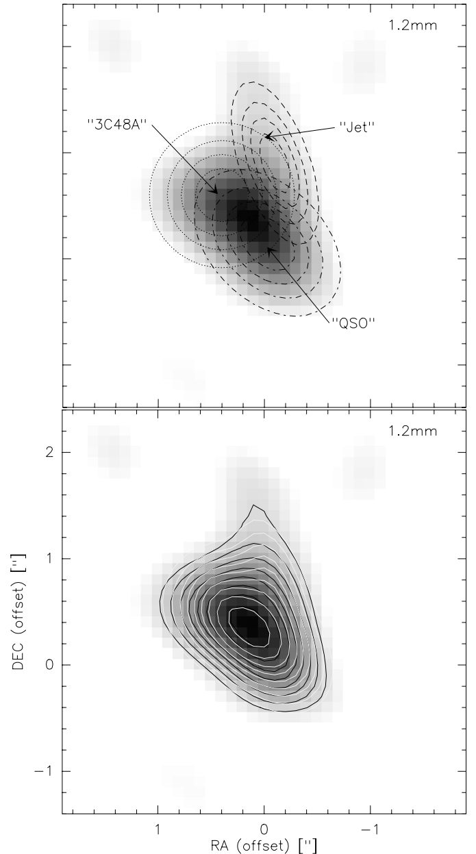
Fig. 4. Upper panel: contours of a triple-Gaussian model: “QSO” (dotted/dashed lines), “jet” (dashed lines), and “3C 48A” (dotted lines). Contours are from 20 to 100% in steps of 20% of the peak fluxes of each component. Lower panel: the sum of the model components (white solid contours), compared with the observed 1.2 mm continuum (grey scale and black solid contours); data and model contours are as in Fig. 2. Data are taken from the 2003 data set only.
