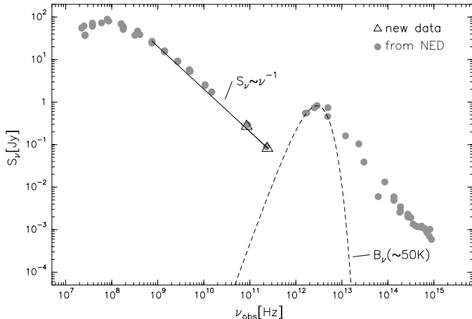
Fig. 3. Flux density spectrum of 3C 48. Grey points are from the NASA/IPAC Extragalactic Database (NED). The triangles at 3.5 mm and 1.2 mm are from our new data, and are the total flux of our continuum fit components. The solid line is a power-law fit to the cm-radio synchrotron emission, and the dashed curve in the infrared (2–10 THz) is a model spectrum for a rest-frame dust temperature of 50 K, a dust \tau = 1 at rest-frame 100\mu\text{m} , and an optically-thin, \nu^4 dependence in the mm range.
