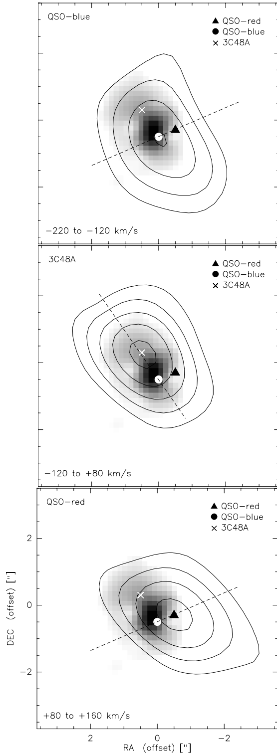
Fig. 10. CO(1–0) integrated over the following ranges (merged 1995 and 2003 data set): Upper: QSO-blue, from -220 to -120 km s ^{-1} ; contours run from (2\sigma)=0.08 to 0.2 Jy beam ^{-1} km s ^{-1} in steps of 1\sigma . Middle: 3C48A, from -120 to 80 km s ^{-1} ; contours run from (3\sigma)=0.42 to 0.98 Jy beam ^{-1} km s ^{-1} in steps of 1\sigma . Lower: QSO-red, from 80 to 160 km s ^{-1} ; contours run from (3\sigma)=0.15 to 0.3 Jy beam ^{-1} km s ^{-1} in steps of 1\sigma . Dashed lines show the cuts on which the pv-diagrams were made. The CO beam is 3.6'' \times 2.5'' . All the CO maps are superposed on the NIR image of Zuther et al. (2004) (grey scale).
