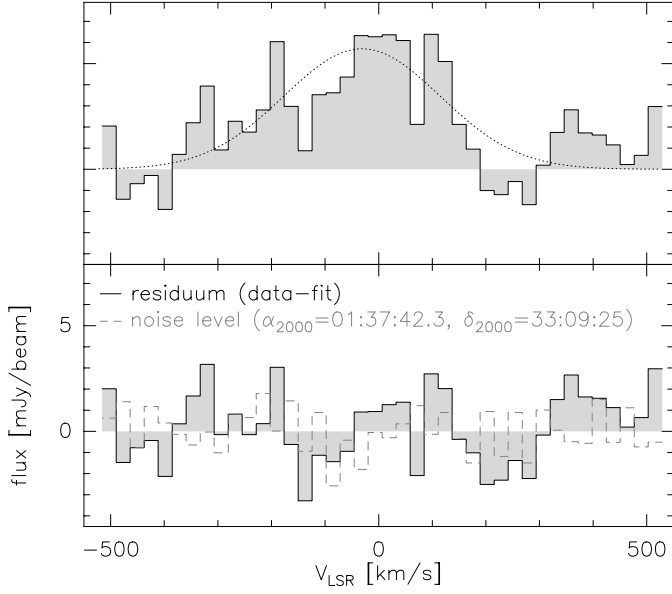
Fig. 7. Upper panel: spectrum at the CO(1–0) centroid in 3C 48 taken from the merged 1995 and 2003 data set (solid histogram), with a Gaussian fit to the data. Lower panel: residual spectrum after subtracting the fit from the data (dotted line). The dashed histogram is a spectrum taken at an off-source position with no CO emission, where the rms noise is 0.9 mJy. The velocity resolution is 26 \text{ km s}^{-1} .
