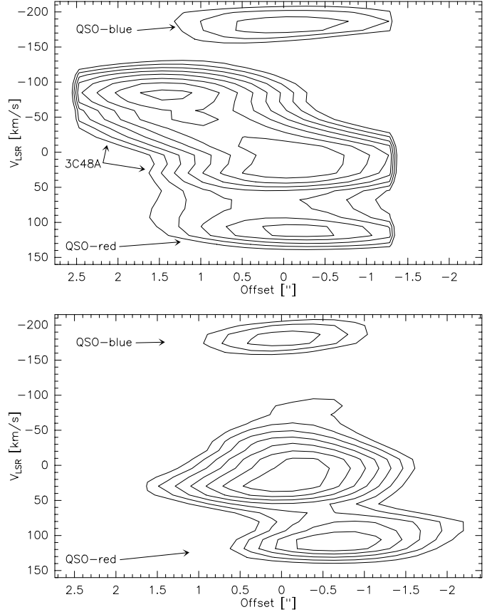
Fig. 9. CO(1–0) position-velocity diagram along the cuts indicated by the dashed lines in Figs. 8 and 10 (merged 1995 and 2003 data set). Contours are from 35% in steps of 5% from the peak. Upper panel: the p-v cut from northeast to southwest, shown in Fig. 8 and in the middle panel of Fig. 10. Lower panel: the p-v cut from southeast to northwest, shown in Fig. 8 and in the upper and lower panels in Fig. 10. The offsets are relative to the position of the CO-QSO-blue component.
