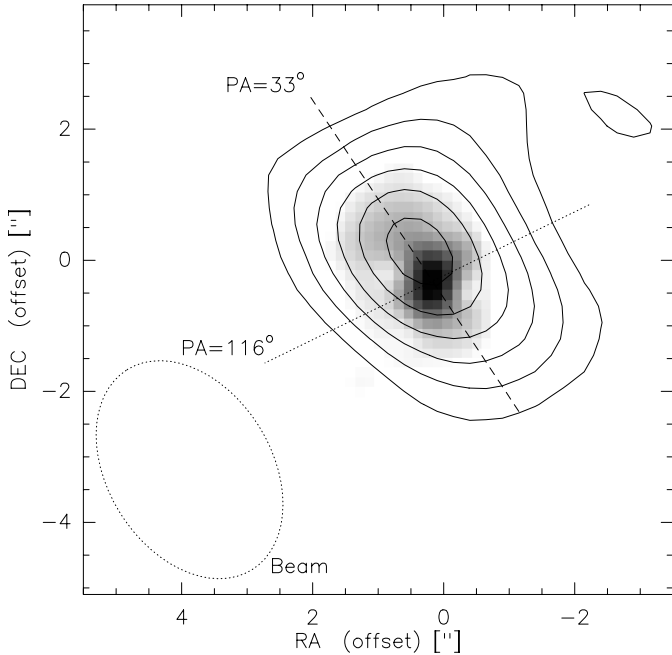
Fig. 8. Integrated CO(1–0) emission of 3C 48 (from -220 \text{ km s}^{-1} to 160 \text{ km s}^{-1} ; merged 1995 and 2003 data). The synthesized beam is indicated in the lower left ( dotted ellipse ). The dashed and dotted lines show the cuts along which the position-velocity diagrams were taken. Contour levels are from (3\sigma)=0.6 to 1.6 \text{ Jy beam}^{-1} \text{ km s}^{-1} by 0.2 \text{ Jy beam}^{-1} \text{ km s}^{-1} . Beam: 3.6'' \times 2.5'' at \text{PA} = 32^\circ . The CO map is superposed on the NIR image of Zuther et al. (2004) ( grey scale ).
