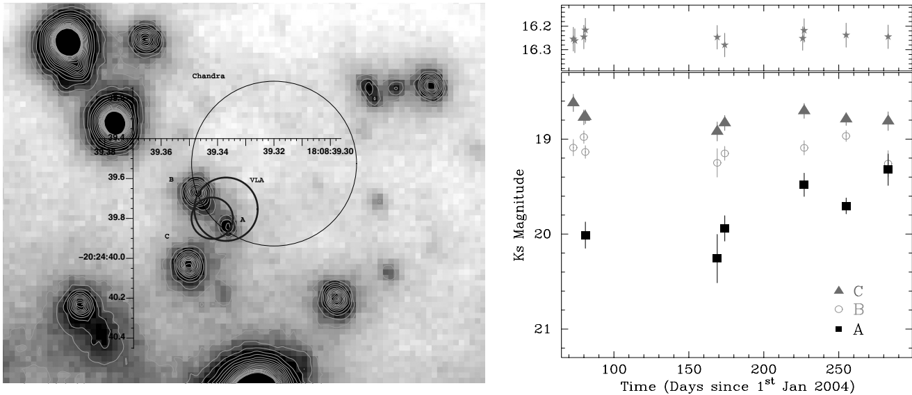
Fig. 1. IR NACO K_s band image ( left panel ; 18th June 2004 dataset) close-up of the 1'.5 \times 1'.5 portion of the sky around the 1\sigma Chandra and VLA uncertainty circles (radius of 0'.3 , 0'.04 and 0'.1 , respectively) with the proposed counterpart marked with A. Coordinates are RA (h m s) and Dec ( ^\circ ' '' ; equinox J2000). Isophotal contour lines are also drawn for clarity. K_s light curves ( right panel ) for a number of selected sources: the proposed counterpart to SGR 1806–20 (A) with two nearby objects ( lower panel ), and the closest reference (isolated and bright) star ( upper panel ) we used for relative photometry among K_s frames. Flux variability is clearly detected only for object A.
