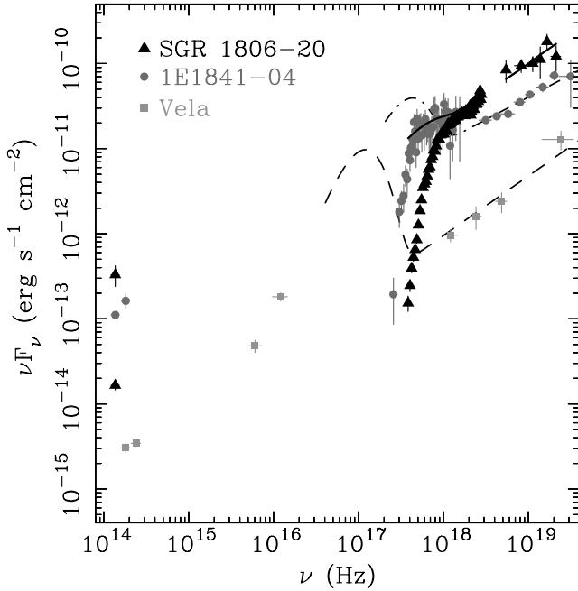
Fig. 2. Broad band energy spectrum of SGR 1806–20 (triangles) and, as a comparison, the AXP 1E 1841–045 (circles) and the radio pulsar Vela (squares). In the case of SGR 1806–20 and 1E 1841–045 high energy data are taken from XMM-Newton (Mereghetti et al. 2005b; referring to 6th October 2004 for SGR 1806–20), Chandra (for 1E 1841–045) and INTEGRAL (Mereghetti et al. 2005a; 21st September–14th October 2004 for SGR 1806–20). Absorbed and unabsorbed IR fluxes ( A_V = 29 \pm 2 , 5th October 2004 NACO observation) are shown in the case of SGR 1806–20, unabsorbed ( A_V = 13 \pm 1 ) IR fluxes are instead reported for the likely candidate of 1E 1841–045 (circles; Israel et al. 2005, in preparation). All the data for Vela are taken from literature (Kaspi et al. 2004, and references therein). Solid curves (continuous, stepped and dot-stepped) are the unabsorbed fluxes for the black body plus power law model used to fit the high energy part of spectra.
