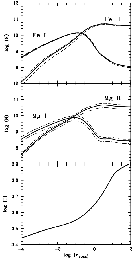
Fig. 3. Atmospheric models for Star # 1665. All models correspond to T_{\text{eff}} = 3945 K \log g = 0.80 . The solid lines refer to an opacity sampling ATLAS 12 model with abundances as provided in Table 2. The dashed lines refer to an ATLAS 9 model computed with a solar-scaled ODF with [M/H] = -0.5 and a microturbulence of 1 \text{ km s}^{-1} . The dash-dotted lines refer to the ionization structure of the ATLAS 9 model computed by WIDTH when the abundances of Table 2 are provided as input. The top panel shows the Fe I and Fe II ions, the middle panel the Mg I and Mg II ions, while the bottom panel displays the temperature structure of the model. The neutral ions show a peak in number densities around \log \tau_{\text{ross}} \sim -1.5 .
