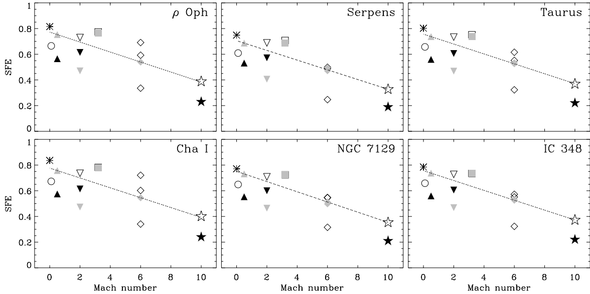
Fig. 3. The star formation efficiency at time \tau plotted versus the Mach number of the models. The symbols are the same as in Fig. 2, circles denote models with M = 0.1 . The dotted lines show a linear fit to the data.
