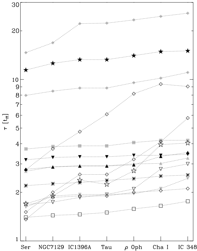
Fig. 2. The time \tau of the best correspondence between models and observations (in units of the global free-fall time \tau_{\text{ff}} ) for the seven investigated clusters. The symbols denote the parameters of the models: \mathcal{M} = 0.5 (triangles), \mathcal{M} = 2 (triangles down), \mathcal{M} = 3.2 (squares), \mathcal{M} = 6 (diamonds), \mathcal{M} = 10 (stars); 1 \leq k \leq 2 (open symbols), 3 \leq k \leq 4 (grey symbols), 7 \leq k \leq 8 (filled symbols). The Gaussian collapse models are displayed as asterisks.
