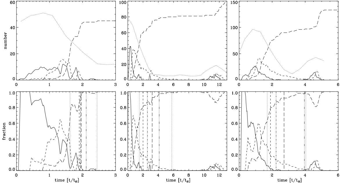
Fig. 1. The temporal evolution of the fractions of YSO classes for three models: M2k4 ( left ), M6k2a ( middle ), and M10k2 ( right ), upper panel : absolute numbers, lower panel : relative numbers. Solid line: Class 0, dashed line: Class 1, long dashed line: Class 2+3, dotted line: prestellar cores (only shown in the upper panel ). The abscissa gives the time in units of the global free-fall time. The zero point of the timescale corresponds to the time when gravity is “switched on”. Note the different intervals covered in the models. The vertical lines in the lower panel indicate the time \tau , when the model shows the best agreement with the observations of Serpens (dotted), NGC 7129 (dashed), Taurus and IC 1396A (dash-dotted), \rho Ophiuchi (long dashes), Cha I (dash-dot-dot-dot), and IC 348 (second dotted line). Because of similar relative YSO numbers, the best-fit evolutionary times for Taurus and IC 1396A are essentially indistinguishable.
