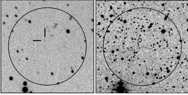
Fig. 1. Left: 6' \times 6' field around the optical afterglow (at the cross point of vertical and horizontal bars) as imaged by ART in I_c band ( 2 \times 60 s). The circle shows the 2.5 radius INTEGRAL error region (Mereghetti et al. 2004). North is up and East is to the left. The narrow elongated object in the middle of the image is a cosmic ray event. Right: the GRB 041218 field in the digitized Palomar Observatory Sky Survey (DSS2 Red) is shown for comparison. A small circle shows the afterglow position.
