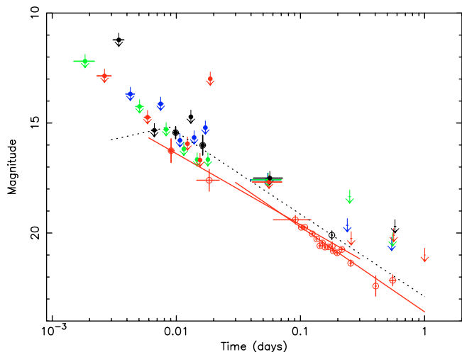
Fig. 2. BVR_cI_c afterglow light curve of GRB 041218. The horizontal axis shows time from GRB onset. Blue, green, red, and black marks show, B , V , R_c , and I_c measurements, respectively. In addition to our measurements (filled circles; arrows mark 2\sigma upper limits), those reported in GCN circulars (Yonetoku et al. 2004; Klotz et al. 2004; Ferrero et al. 2004; Monfardini et al. 2004; D’Avanzo et al. 2004; Halpern et al. 2004; Cenko et al. 2004; Mirsa & Pandey 2004) are plotted with open circles (detections) or arrows (upper limits). See discussion in text for the black and red lines.
