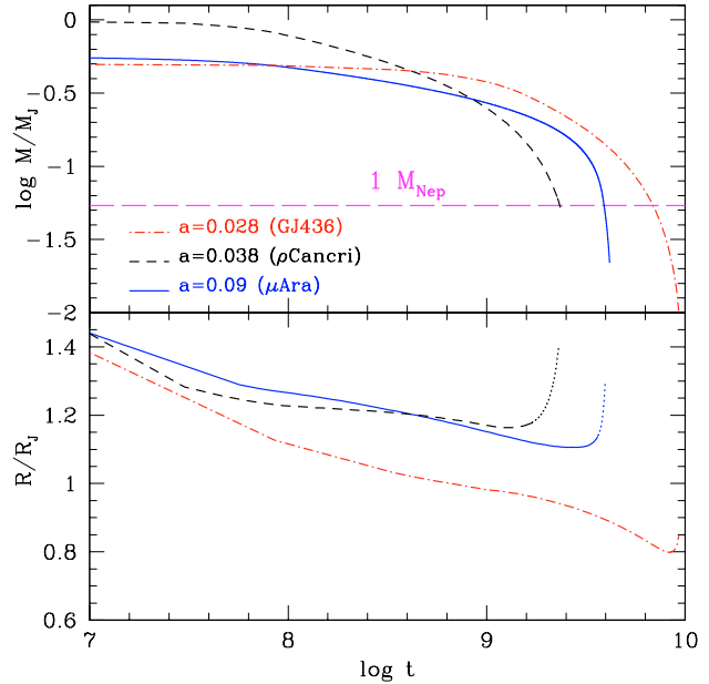
Fig. 2. Evolution of evaporating giant planets reaching a Neptune-mass (indicated in the top panel by the long-dashed line, in Jupiter-mass units M_J ) within a few Gyr. Three planet-star cases are shown for: the G5 star \mu Ara (Santos et al. 2004) (solid), the G8 star \rho^1 Cancri (McArthur et al. 2004) (dashed), and the M 2.5 star GJ 436 (Butler et al. 2004) (dash-dotted). The planet's orbital separation a (in AU) for each system is indicated in the upper panel.
