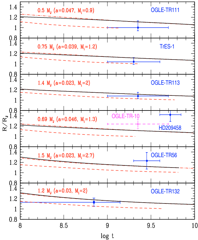
Fig. 1. Evolution of the radius (in R_J ) for currently known transiting planets. The incident stellar flux contribution, F_{\text{inc}} , increases from top to bottom. The measured mass and orbital separation are indicated in each panel. The curves correspond to evolutionary models for three cases: without irradiation (dashed lines), with irradiation effects on the thermal structure but no evaporation (dash-dotted lines), and with irradiation and evaporation effects (solid lines). For the latter cases, the initial mass M_i is also indicated in each panel. Note that in most cases the dash-dotted (no evaporation) and solid (evaporation) lines are undistinguishable (see text).
