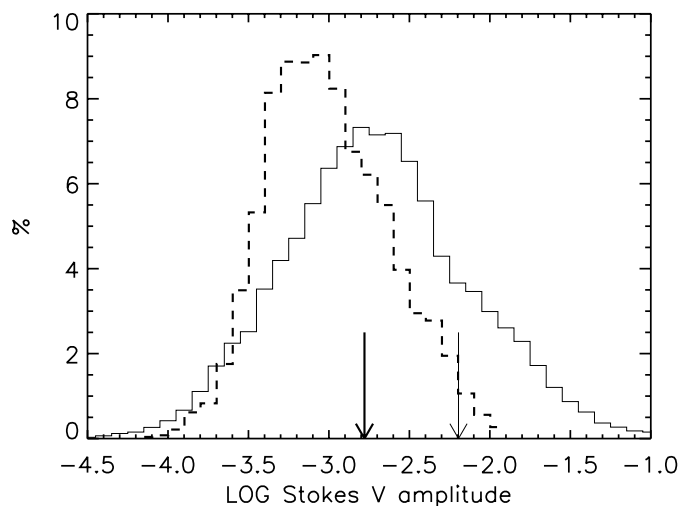
Fig. 1. Histograms of the amplitudes of Stokes V of Fe I 630.2 nm in the \langle B \rangle = 20 \text{ G} simulation snapshot. Solid line: original resolution; dashed line: reduced resolution. Arrows indicate the mean values.
