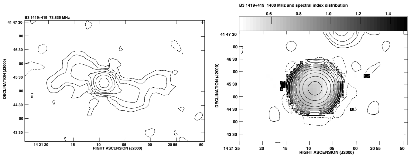
Fig. 7. B3 1419+419: left : 74-MHz map, contour levels: -0.2, 0.2, 0.4, 0.8, 1.6, 3.2, 6.4, 12.8 Jy/beam; right : spectral index distribution (grey), NVSS flux densities (contours), contour levels: -1, 1, 2, 4, 8, 16, 32, 64, 128, 256, 512, 1024, 2048 mJy/beam.
