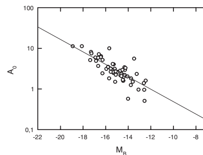
Fig. 3. The linear diameter A_0 is given versus the absolute blue magnitude of all galaxies of our sample. The solid line represents the sample of nearby galaxies (KKHM). The range covered by both coordinates is the total range covered by the comparison sample.
