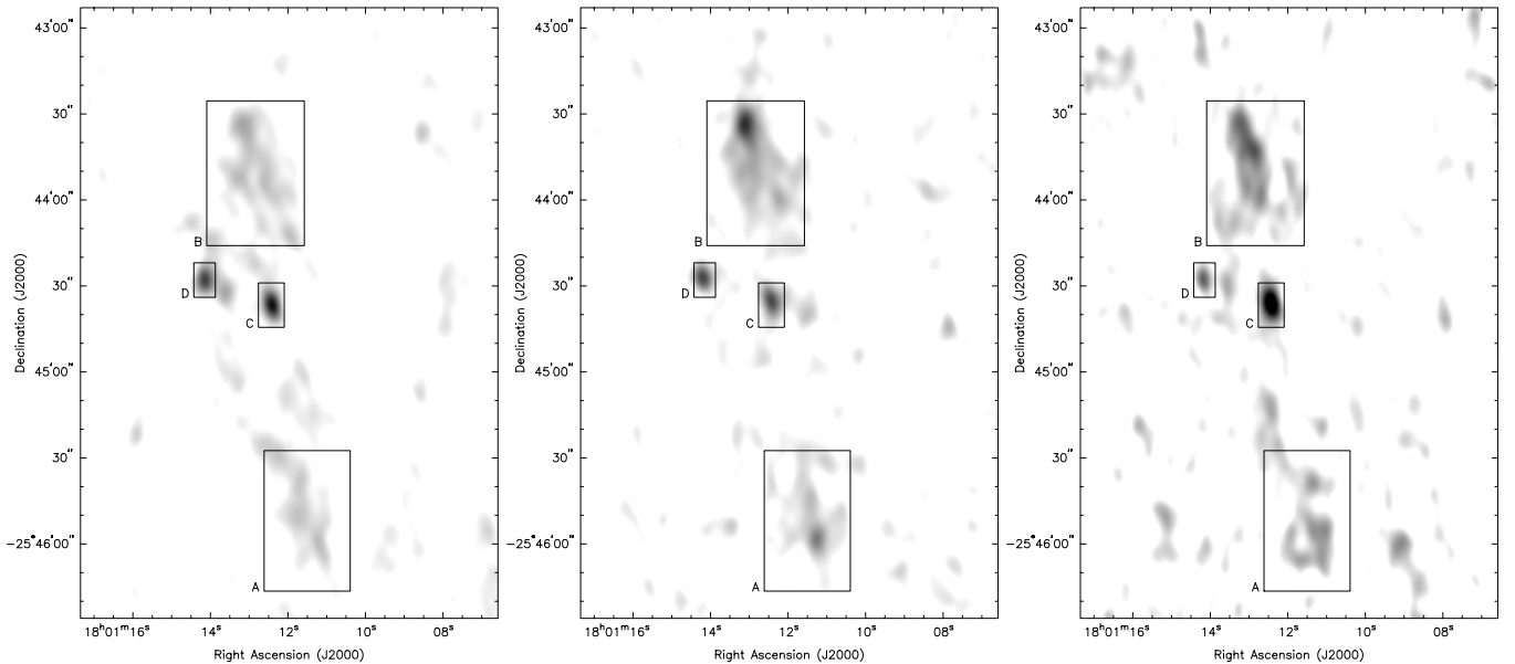
Fig. 1. Greyscale images of the GRS 1758–258 lobes at the three frequencies used in the paper: 1.4 GHz ( left ), 4.9 GHz ( centre ) and 8.4 GHz ( right ). All three images have the same resolution, 9.2 \times 5.8 arcsec. The greyscale ranges from the 2\sigma level of the off-source noise to 0.5 \text{ mJy beam}^{-1} (1.4 GHz), 0.2 \text{ mJy beam}^{-1} (4.9 GHz) and 0.15 \text{ mJy beam}^{-1} (8.4 GHz). Boxes show the extraction regions used for the four source components discussed in the paper. Component C is identified with the X-ray source.
