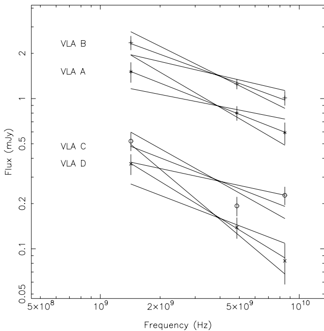
Fig. 2. The flux densities and best power-law fits of the components of GRS 1758–358. The solid lines show the best-fitting lines and the 90% confidence limits on the slope.
