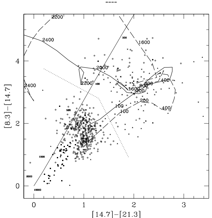
Fig. 4. Evolutionary tracks of an oxygen-rich star in the post-AGB phase. Evolution time is plotted next to the curves and is counted in years. The two curves correspond respectively to mass loss rates of 2.1 \times 10^{-5} M_\odot/\text{year} (model a, continuous line) and 5.2 \times 10^{-6} M_\odot/\text{year} (model b, dashed line). The symbols are the same as in Figs. 2 and 3 but have been shrunk to make the curves clearer.
