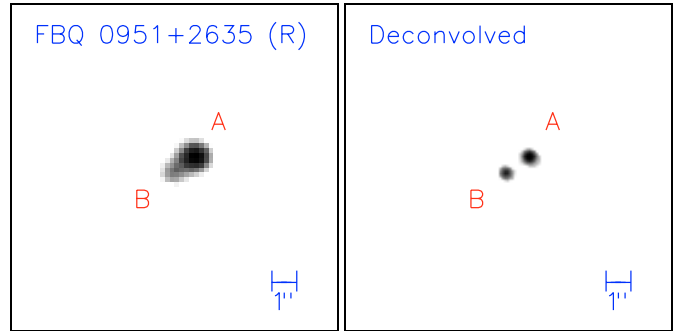
Fig. 2. Left: stacked R -band image of a 12'' \times 12'' region centered on FBQ 0951+2635. The seeing is \sim 1''.2 and the total exposure time is \sim 8.3 h. Right: deconvolved image ( FWHM = 0''.28 ) obtained from the simultaneous deconvolution of 49 frames. North is up and east to the left.
