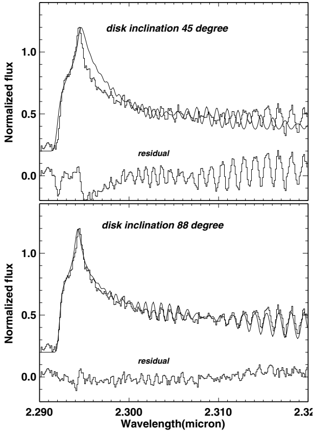
Fig. 2. Fits to the CO first bandhead ( v = 2-0 ). In the upper panel the thin line corresponds to the normalized observed spectrum while the thick line is the best fit if the disk is viewed at an inclination of 45^\circ . The lower plot is the residual of the fit. The lower panel shows the best fit obtained with a disk viewed at an inclination of 88^\circ . The complete set of parameters is reported in Table 1.
