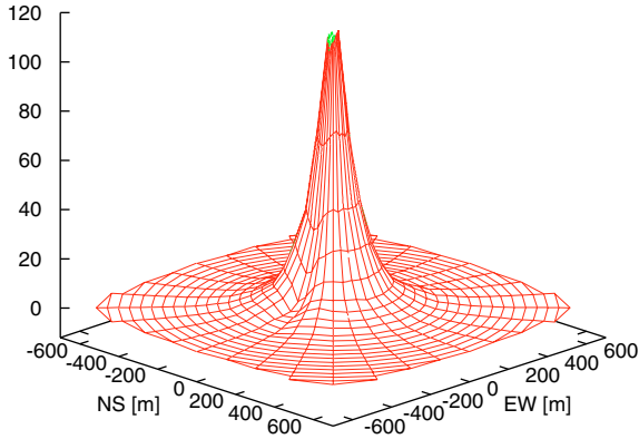
Fig. 24. Pattern of the maximum filtered electric field amplitude (in \mu\text{V m}^{-1} ) emitted by the maximum of a 10^{17} eV air shower consisting of 10^8 particles at a height of 4 km for a 0.5 Gauss 70^\circ inclined magnetic field, a broken power-law particle energy distribution and a statistical distribution of track lengths.
