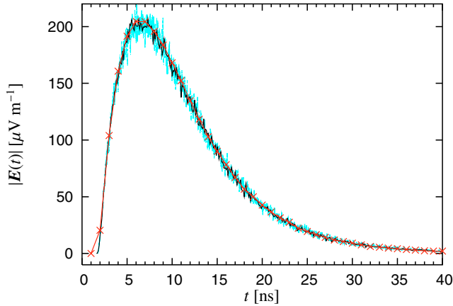
Fig. 11. Raw pulse from a shower slice calculated with different grid- ding strategies and resolutions. Solid with points: simple grid 10^{-9} s, solid black: simple grid 10^{-10} s, light coloured: economic grid 10^{-12} s.
