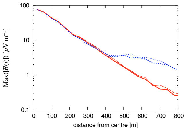
Fig. 12. Changes introduced by the smart sampling algorithm in the radial emission pattern of the rectangle-filtered maximum pulse ampli- tude for emission from the shower maximum. Thin lines: dense equidistant sampling, thick lines: smart sampling; solid: to the north, dashed: to the west.
