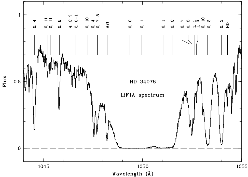
Fig. 1. Portion of the January 2000 LiF1A spectrum in units of 10^{-11} erg s ^{-1} cm ^{-2} Å ^{-1} near strong H _2 ( J = 0, 1, 2 ) lines from the (4–0) Lyman band. \nu and J values for the lower level of each H _2 transition involved are given. The features indicated illustrate the variety of excited H _2 levels from which absorption is detected. The identification of the feature noted “4, 2 ?” is uncertain (see text in Sect. 2.3).
