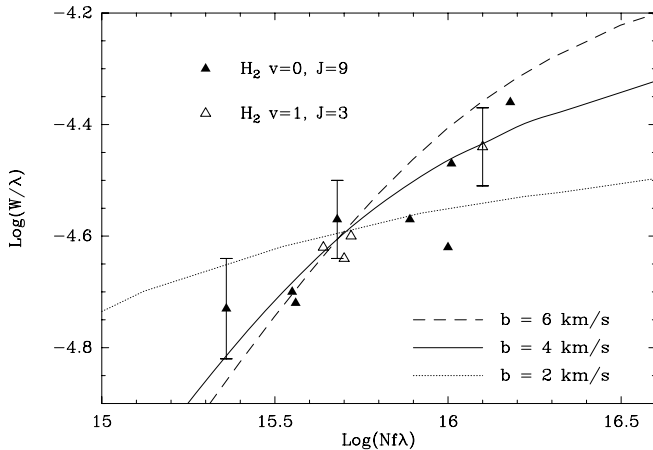
Fig. 3. Curve of growth for H 2 transitions from the v = 0 , J = 9 and the v = 1 , J = 3 levels (filled and empty triangles respectively). The horizontal scale is appropriate for b = 4 \text{ km s}^{-1} ; the slopes of the curve of growth corresponding to b = 2 and b = 6 \text{ km s}^{-1} are indicated (dotted and dashed line, respectively). A few representative 1\sigma error bars are given.
