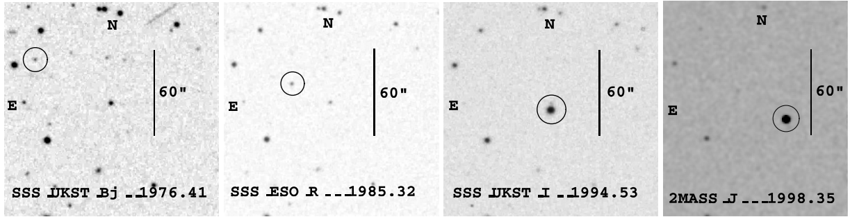
Fig. 1. Finding charts of SSSPM J1444–2019 (circled) at different epochs clearly illustrating its extremely large proper motion. The different passband data are sorted according to the epochs at which they were taken, from blue and red SSS plates to the most recent epoch 2MASS J band image, and also demonstrate the very red optical and optical-to-infrared colours of the object (see also Table 1). North is up and East left.
