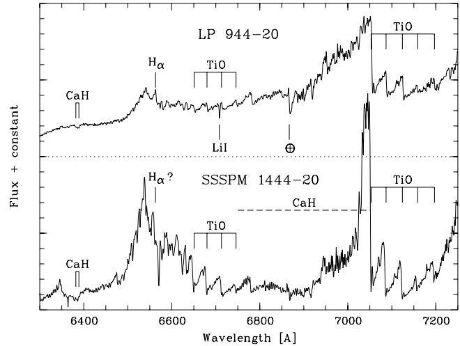
Fig. 3. FORS2 spectra of SSSPMJ1444–2019 and the brown dwarf LP944-20. The spectral region employed in the Gizis (1997) subdwarf classification scheme is shown. The Li absorption line at 6708 \text{ \AA} in LP944-20 and some of the sharp spectral features (mainly TiO) used in the radial velocity determinations are marked. Telluric absorption is indicated by a circled plus sign.
