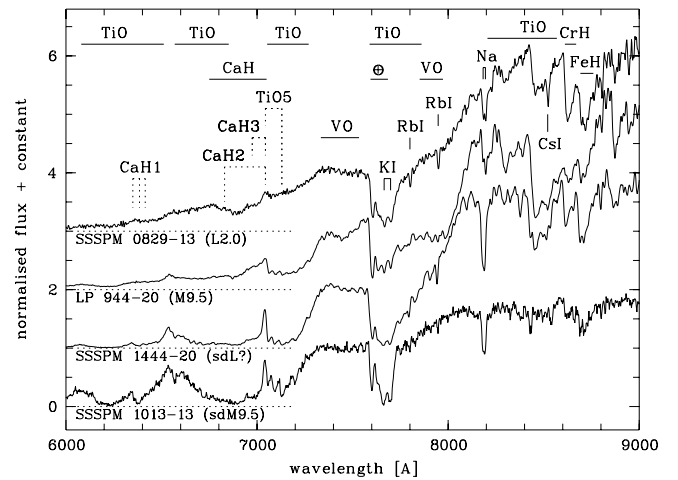
Fig. 2. Optical spectra taken with EFOSC2 on the ESO 3.6-m telescope for SSSPM J1444–2019, LP 944-20, and SSSPM J0829–1309, along with an NTT/EMMI spectrum of the latest known M-type subdwarf (sdM9.5) SSSPM J1013–1356 (Scholz et al. 2004). The spectra are normalised at 7500 Å. Key spectral features of M and L (sub)dwarfs are labeled. Also shown are the spectral regions defining the spectral indices TiO5, CaH1, CaH2, and CaH3 used in the Gizis (1997) subdwarf classification scheme. Uncorrected telluric absorption is indicated by the circled plus sign.
