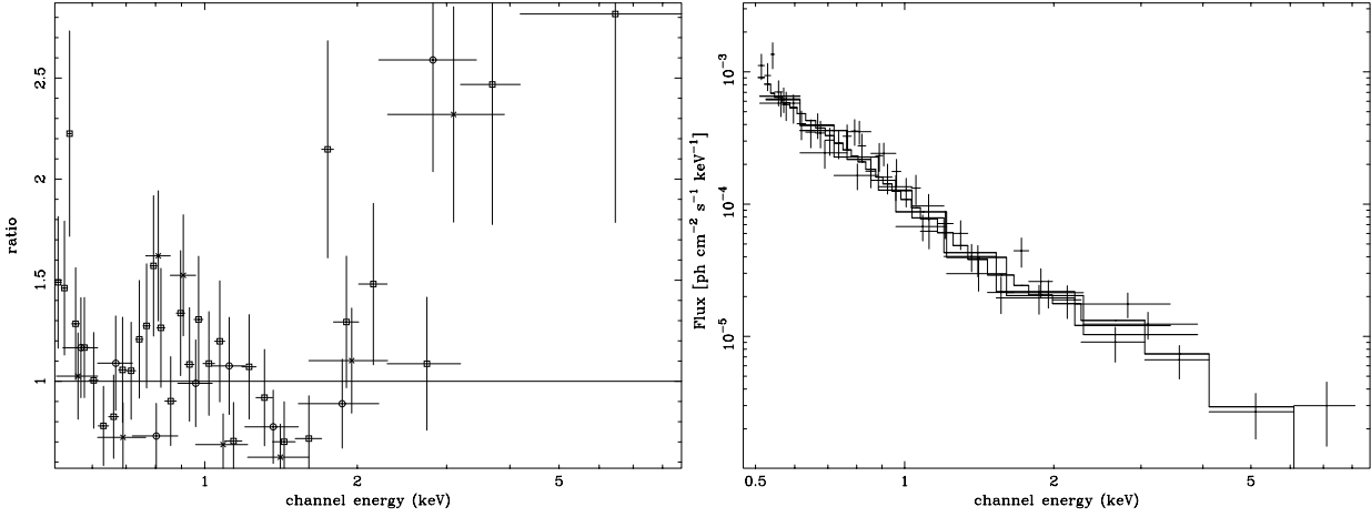
Fig. 3. ( left ) Ratio data/model of the EPIC data of SD1 fitted with only a power law absorbed by the Galactic column. Circles are MOS1 data, crosses are MOS2 data, and squares are PN data. The soft and hard excesses are clearly visible. Data are rebinned for clarity. ( right ) Unfolded spectrum of SD1 with the best fit model (partial covering).
