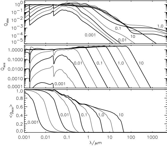
Fig. 4. Derived optical properties of spherical iron grains. Shown are the absorption coefficients Q_{\text{abs}}(\lambda, a) , scattering coefficients Q_{\text{sca}}(\lambda, a) , and the scattering parameter g_{\text{sca}}(\lambda, a) = \langle \cos(\theta) \rangle at 25 K for various grain radii from 10 Å to 10 μm with a difference in radius of \Delta \log a [\mu\text{m}] = 0.5 . Thick lines are labeled with the corresponding grain radii in microns.
