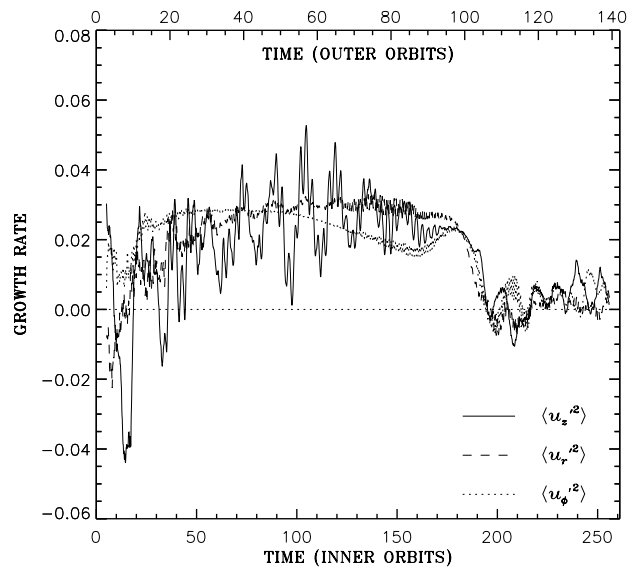
Fig. 7. The growth rate for the square of the velocity fluctuations for model S. The graph is smoothed and does not show the short-term oscillations indicated by Fig. 5. The growth rate is given in units of \Omega(r_{\max}) .
