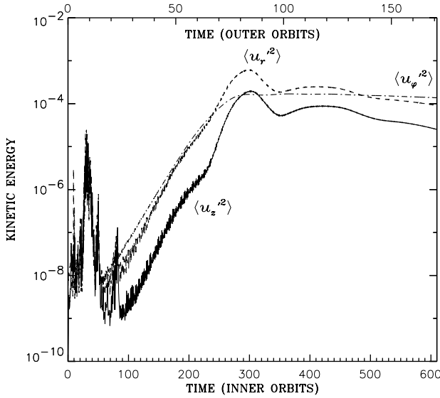
Fig. 8. Energies in velocity fluctuations for model L.
