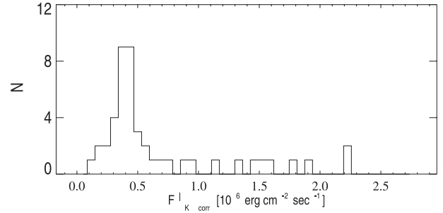
Fig. 10. Histogram of the chromospheric-activity levels in the sample of stars from Pasquini (1992).
