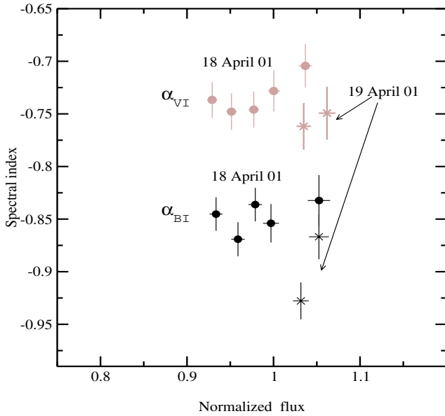
Fig. 6. B - I (filled black circles and crosses) and V - I (grey filled circles and crosses) spectral indices vs the B + I and V + I normalized source flux for the 2001 observations. The data have been smoothed out using the same bin size as with the respective light curves in Fig. 4.
