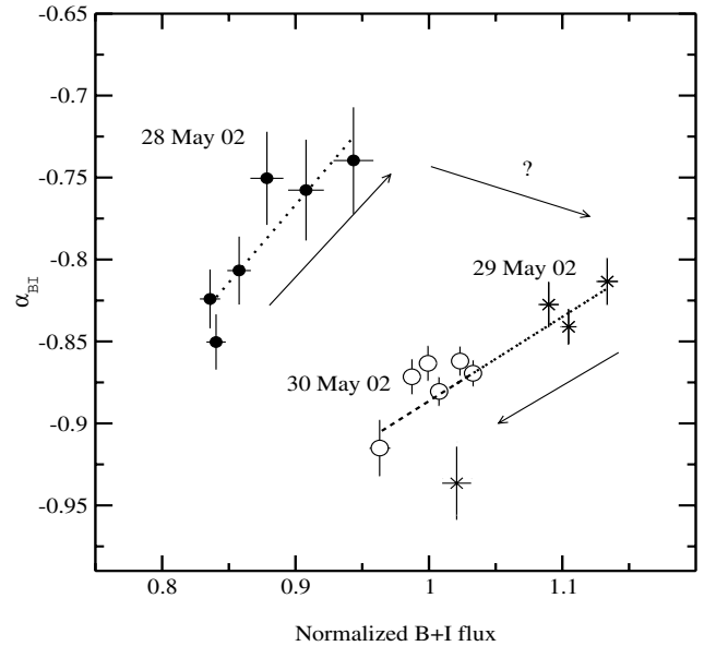
Fig. 5. B - I spectral index vs. the B + I normalized flux for the 2002 observations. For clarity reasons, we have smoothed the data using the same bin size that we have used for the respective light curves in Fig. 3. The dotted lines show the best linear model fit to the data, while the arrows indicate the flux variability trend (i.e. flux increase or decrease) during the observations (see text for details).
