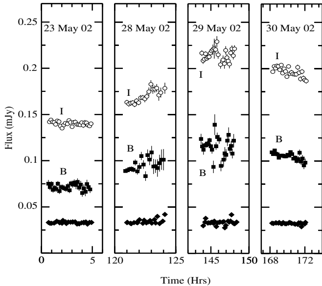
Fig. 2. B and I band light curves during the 2002 observations. Time is measured in hours from 18:00 UT on May 23, 2002. As before with Fig. 1, the small filled diamonds show the B band light curve of the comparison star 2 (shifted to a mean of \sim 0.033 mJy).
