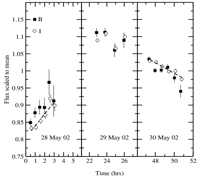
Fig. 3. B and I band light curves in 2002 (filled squares and open circles, respectively) normalized to their average flux level. Time is measured in hours from the beginning (plus half an hour) of the May 28 B band observations. In order to reduce the experimental noise, we have smoothed the May 28, 29 and 30 light curves using a bin size of 3, 6, and 4, respectively.
