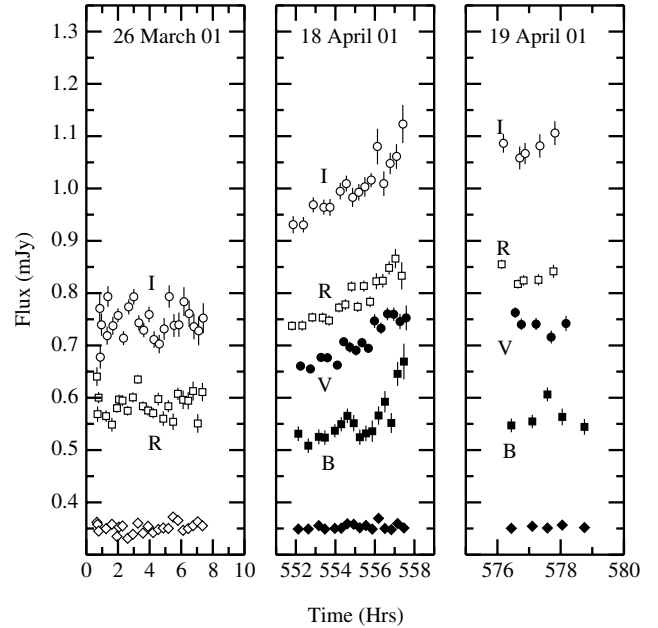
Fig. 1. B , V , R , and I band light curves during the 2001 observations. Time is measured in hours from 19:00 UT on March 26, 2001. The small filled diamonds below the B band light curve of S4 0954+658 show the B band light curve of the comparison star 2 (open diamonds in the left panel show the R band light curve of the same star). For clarity reasons, the standard star light curves are shifted to the same level of \sim 0.35 mJy.
