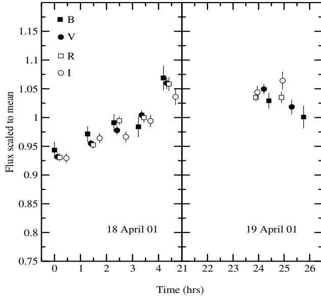
Fig. 4. Same as Fig. 3 for the April, 2001 light curves (filled squares, filled circles, open squares, and open circles show the B , V , R , and I band light curves, respectively). The light curves have been smoothed out using a bin size of 3, except from the last point where a bin size of 2 was used. Time is measured in hours from the start of the April 18, B band observations.
