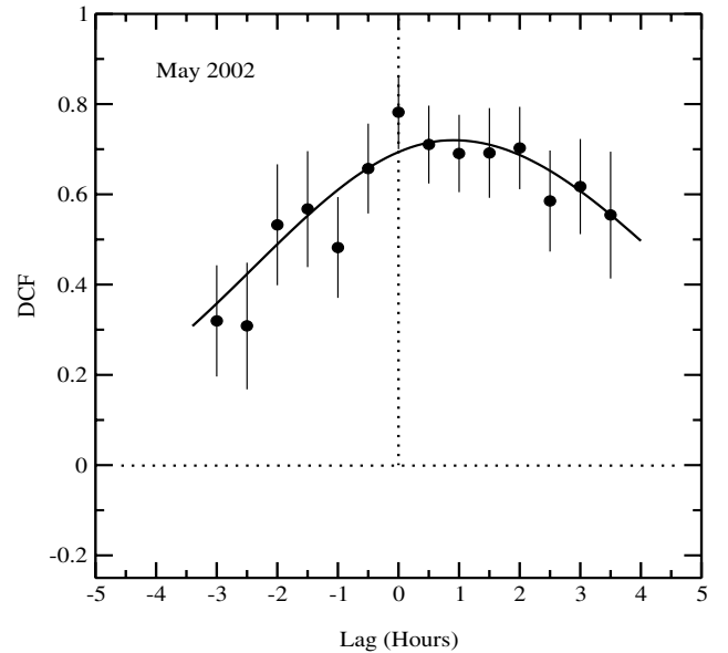
Fig. 7. The Discrete Correlation Function between the B and I band light curves during the late May 2002 observations. Significant correlation at positive lags means that the B band variations are leading the I band. The solid line shows the best fitting Gaussian model to the data.
