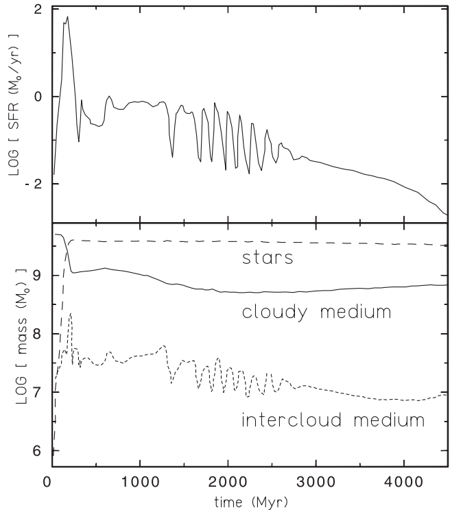
Fig. 5. Star-formation rate ( upper panel ) and masses ( lower panel ) of the 5 \times 10^9 M_{\odot} model from a 3\sigma fluctuation. See text for discussion. For comparison with Fig. 4 notice the different time axes!
