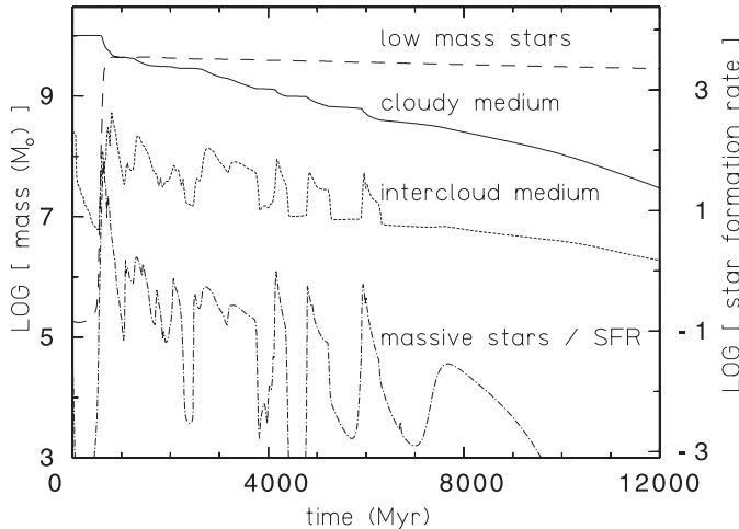
Fig. 7. The temporal evolution of mass distributions (left scale) in a 10^{10} M_{\odot} spherically symmetric galaxy originating from a 1\sigma density fluctuation. While low-mass stars (dashed line), cloudy interstellar medium (thick full line) and intercloud medium (thin dotted line) are drawn individually, the massive star line (dash-dotted) represents simultaneously the star-formation rate (right scale in M_{\odot} \text{ yr}^{-1} ). Reduction of the total mass due to a galactic wind is discernible from the cloudy medium. It coincides temporarily with the peak star-formation rate.
