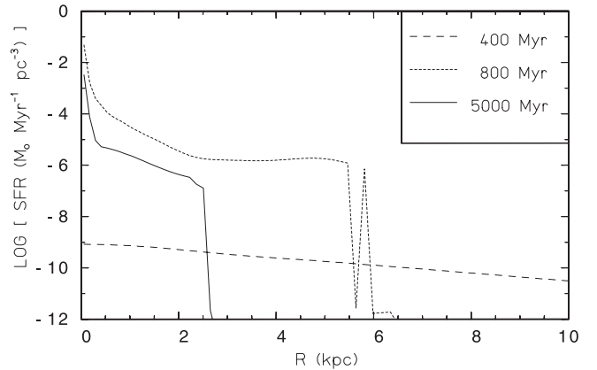
Fig. 8. Radial distribution of the star-formation rate at different times during the evolution of the same 10^{10} M_{\odot} model as in Fig. 7. The radial concentration of the star-forming region is perceivable.
