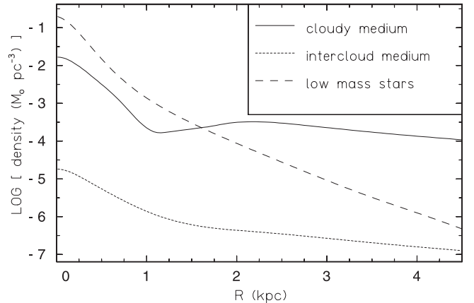
Fig. 2. Radial density distribution of cloudy and intercloud medium as well as low-mass stars after an age of 10 Gyr of the same 10^9 M_{\odot} model as in Fig. 1.
