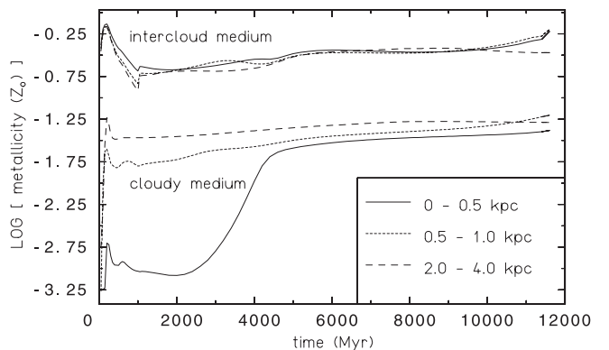
Fig. 3. Temporal evolution of the metallicity of cloudy (lower curves) and intercloud medium (upper lines) at different radial bins of the same 10^9 M_{\odot} model as in Fig. 1.
