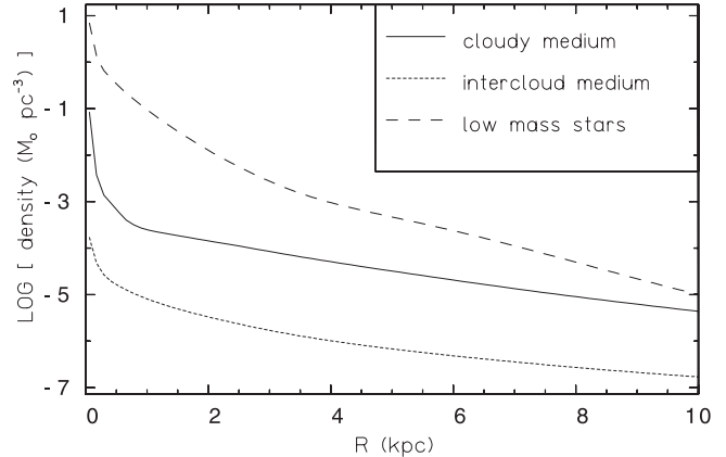
Fig. 11. Radial density distribution of cloudy and intercloud medium as well as low-mass stars after an age of 10 Gyr of the same 10^{10} M_{\odot} model as in Fig. 7.
