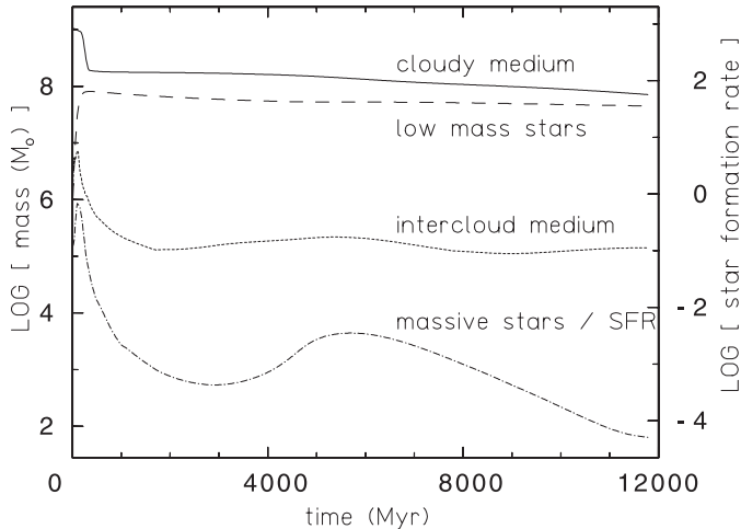
Fig. 1. The temporal evolution of mass distributions (left scale) in a 10^9 M_{\odot} spherically symmetric galaxy originating from a 1\sigma density fluctuation. While low-mass stars (dashed line), cloudy interstellar medium (thick full line) and intercloud medium (thin dotted line) are drawn individually, the massive star line (dash-dotted) represents simultaneously the star-formation rate (right scale; given in M_{\odot} \text{ yr}^{-1} ). Reduction of the total mass is discernible from the cloudy medium.
