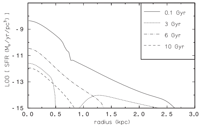
Fig. 6. Radial distribution of the star-formation rate at different times during the evolution of the same 5 \times 10^9 M_{\odot} model as in Fig. 5. The radial concentration of the star-forming region is discernible.
