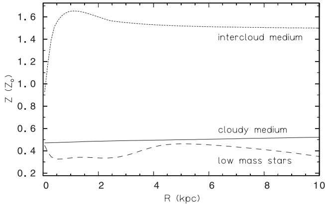
Fig. 12. Radial metallicity distribution of cloudy and intercloud medium as well as low-mass stars after an age of 10 Gyr of the same 10^{10} M_{\odot} model as in Fig. 7.
