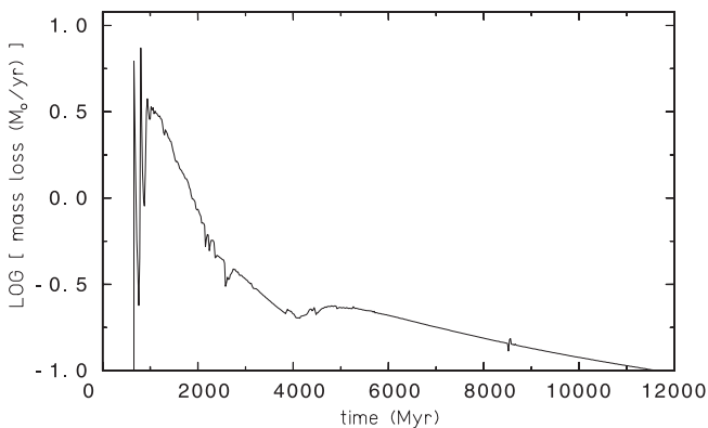
Fig. 10. Same as Fig. 9 but for a 10^{10} M_{\odot} 1\sigma galaxy model with a 10% drag coefficient (see text).
