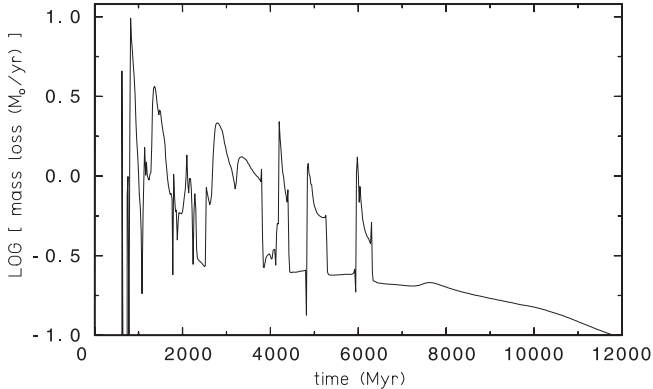
Fig. 9. Time-dependence of the rate of unbound mass with respect to the gravitational potential of the same 10^{10} M_{\odot} model as in Fig. 7. For discussion see text.
