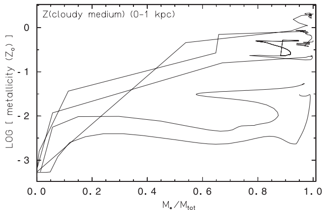
Fig. 13. Evolutionary tracks of the total metallicity Z of the cloudy medium within the inner 1 kpc of the 5 models presented in this paper with increasing stellar mass fraction after 10 Gyr. From lowest to uppermost curve: 10^9 M_{\odot} , 1\sigma ; 10^9 M_{\odot} , 3\sigma ; 5 \times 10^9 M_{\odot} , 1\sigma ; 5 \times 10^9 M_{\odot} , 3\sigma ; and 10^{10} M_{\odot} , 1\sigma .
