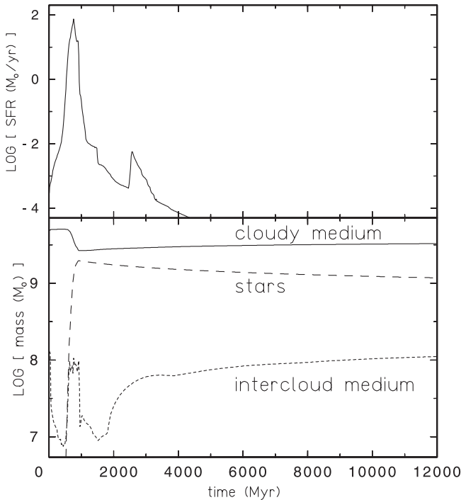
Fig. 4. Star-formation rate ( upper panel ) and masses ( lower panel ) of the 5 \times 10^9 M_{\odot} model from a 1\sigma fluctuation. Remarkably the gas fraction remains dominant although it cannot produce further stars. 40% of the mass is expelled by a galactic wind.
