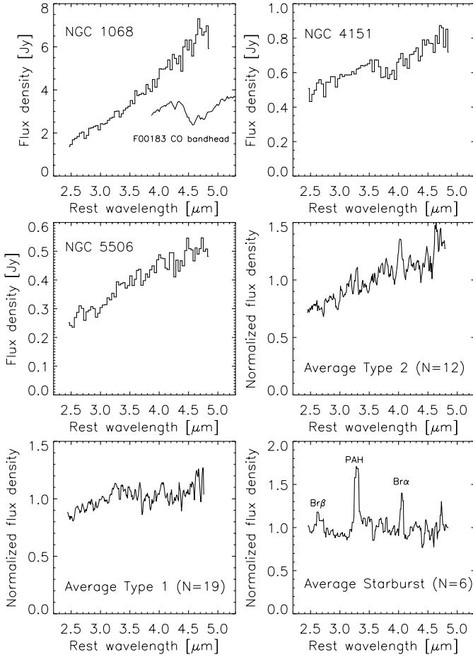
Fig. 1. ISOPHOT-S low resolution 2.5–5 \mu\text{m} spectra of AGN. We show three examples of good S/N spectra, plus averages for type 1 and type 2 Seyferts. These averages include fainter spectra, all normalized to median flux 1 in the observed range before averaging. They give equal weight to all objects irrespective of flux and S/N. A starburst spectrum is shown for comparison and to identify features also seen in some of the AGN spectra. In the top left panel, a scaled spectrum of IRAS F00183-7111 (Spoon et al. 2004) is included for comparison.
