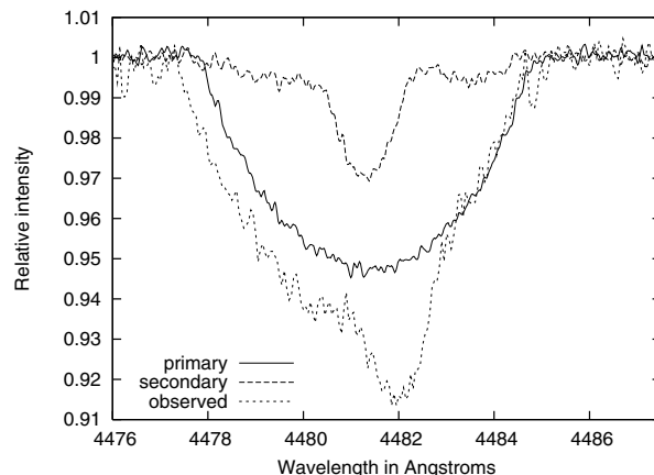
Fig. 2. Disentangled lines of Mg II centered on the systemic velocity. Full line: primary; broken line: secondary. Dotted line: spectrum observed in 1995 near quadrature, at phase \phi \sim 0.1 .
