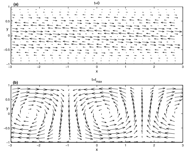
Fig. 6. The flow field \mathbf{u} = (u, v, 0) of the optimal disturbance at t = 0 a ); and at the time of maximum amplification, t = t_{\max} b ); at \text{Re} = 1500 , \text{Ro} = 2/3 , \alpha = 1.2 and t_{\max} = 10.11 .
