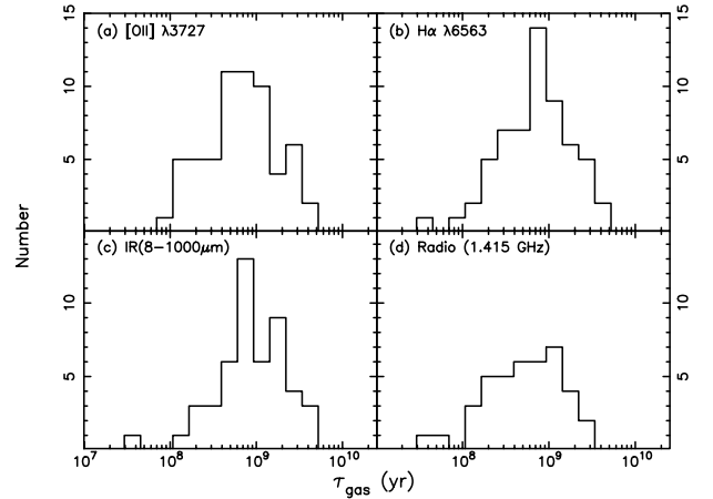
Fig. 6. The gas depletion time-scale of BCGs from H\alpha , [OII]\lambda 3727 emission lines, far-infrared, and radio luminosities. The typical gas depletion time-scale of BCGs is about a few billion years.
