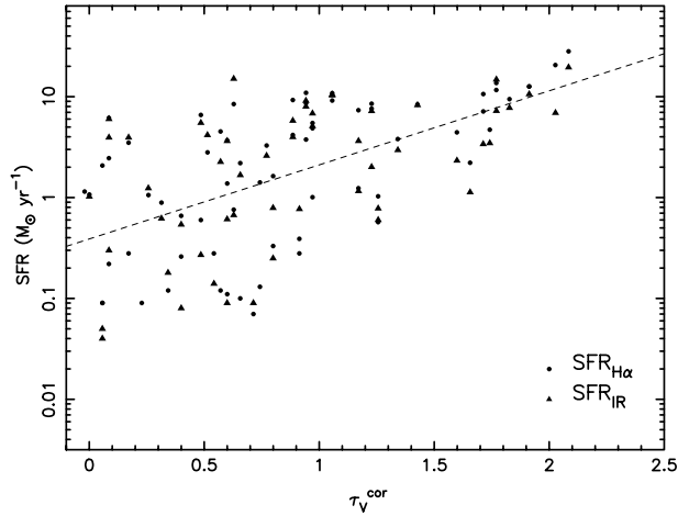
Fig. 8. The dust extinction traced by the Balmer decrement versus the SFR. \tau_V^{\text{cor}} were calculated from the F_{H\alpha} and F_{H\beta} fluxes where the underlying stellar population absorption were subtracted.
