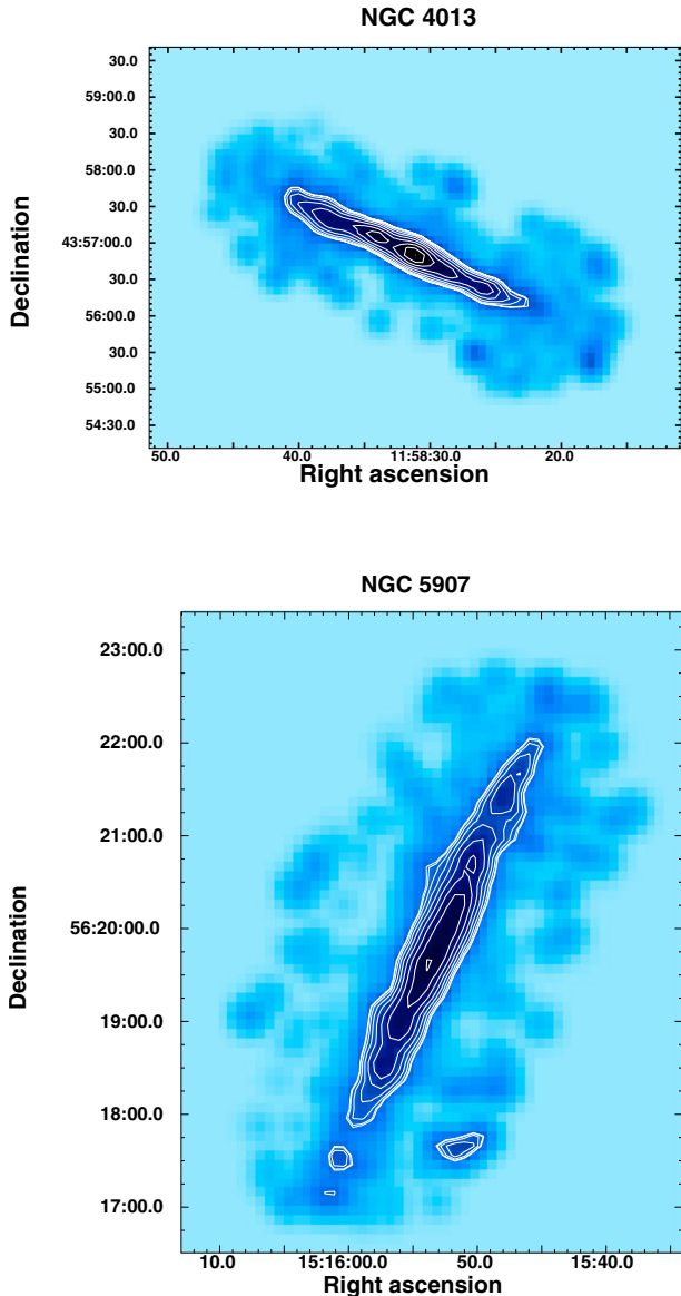
Fig. 1. NGC 4013 ( top ) and NGC 5907 ( bottom ) observed in the 850\ \mu\text{m} continuum with SCUBA. Both the background image and the contours refer to emission at 850\ \mu\text{m} . For NGC 4013 the contour levels are at 10.0, 10.4, 11.4, 13.3, 15.9, 19.2, 23.3, 28.1, 33.7 and 40.0\ \text{mJy}/16'' beam while for NGC 5907 the contour levels are at 20.0, 20.8, 23.4, 27.8, 33.8, 41.6, 51.1, 62.3, 75.3 and 90.0\ \text{mJy}/16'' beam. In both cases the first contour level is at the 3\ \sigma level and the beam size is 16'' ( FWHM ). Coordinates are in epoch 2000.
