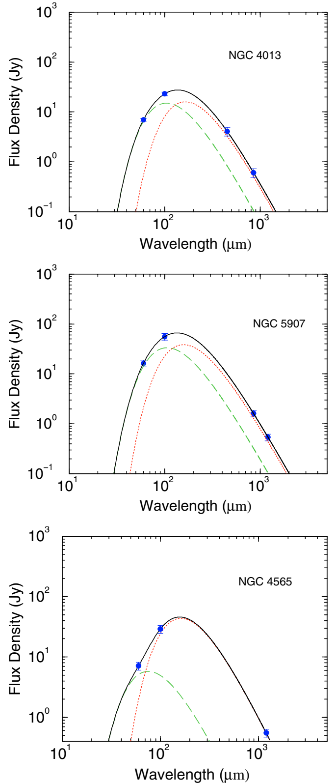
Fig. 3. Flux densities for NGC 4013, NGC 5907 and NGC 4565 as observed by IRAS ( 60 and 100 \mu\text{m} ), SCUBA ( 450 and 850 \mu\text{m} ) and IRAM ( 1.2 \text{ mm} ). In each case, the thermal spectrum has been fitted by the sum of a warm and cold dust component (dashed and dotted lines respectively). The total SED is given by the solid curve. The proportion of dust in each of the warm and cold components, as well as their associated temperatures, are given in Table 3.
