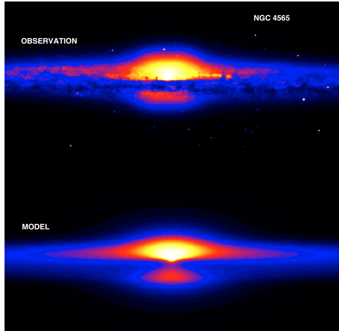
Fig. 2. Radiation transfer modelling of NGC 4565 in the V -band. The real galaxy, as observed by Howk & Savage (1999), is shown at the top whilst the corresponding image generated by our radiation transfer simulation is situated at the bottom.
