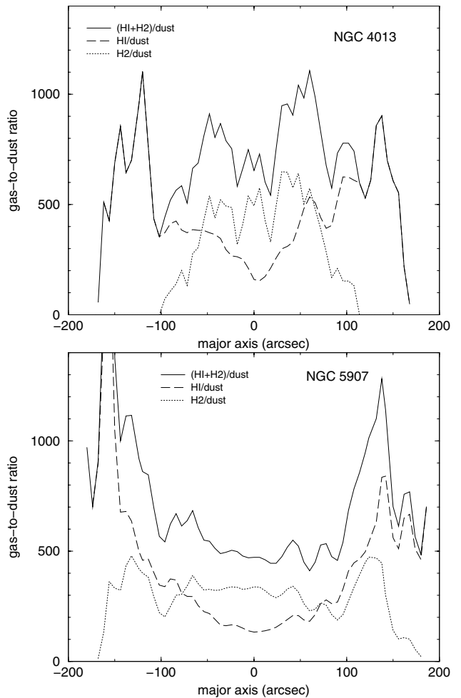
Fig. 7. The gas-to-dust ratio along the major axes of NGC 4013 and NGC 5907. The CO line has been converted to a \text{H}_2 column density assuming X = 2 \times 10^{20} \text{ cm}^{-2} \text{ K km s}^{-1} . The dust column density follows from the submm emissivities derived in Sect. 6 of this work.
