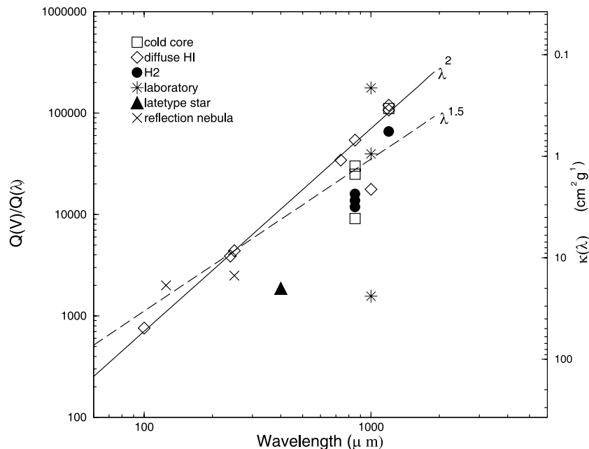
Fig. 5. Emissivity Q(\lambda) of astrophysical dust in the far-infrared, submm and millimeter wavebands. The plot depicts the values collated in Table 4 employing identical markers for similar astrophysical environments. The estimates that we derive for NGC 4013, NGC 4565, NGC 5907 and NGC 891 (the latter in Alton et al. 2000) have been attributed to dust residing in molecular gas clouds (solid circles). The dashed and dotted lines correspond to a wavelength dependency for the emissivity which varies as \beta = 2.0 and \beta = 1.5 respectively ( Q \propto \lambda^{-\beta} ). The lines have been set to pass arbitrarily through the frequently-cited model value of Draine & Lee (1984) at 250 \mu\text{m} .
