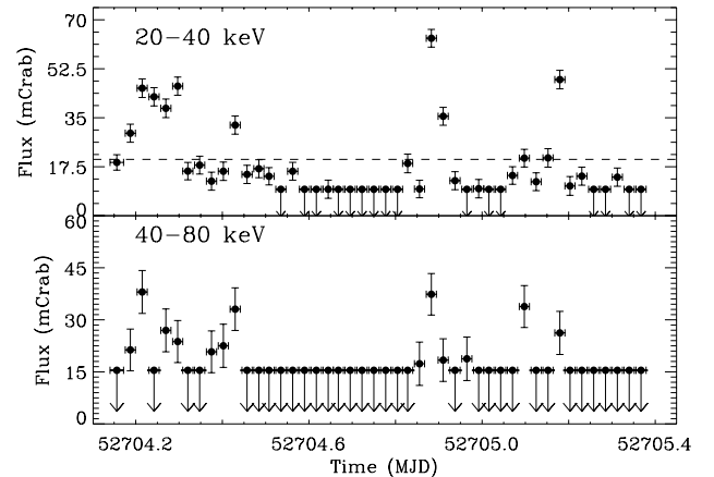
Fig. 2. The 20–40 keV ( top ) and 40–80 keV ( bottom ) ISGRI lightcurves. Each symbol represents a science window. The 3-sigma upper limits are denoted with an arrow. The dashed line in the upper panel indicates the 20 mCrab level.
