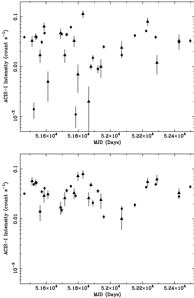
Fig. 3. Long term lightcurve from observations c1–c35 of r2-3 (top) and r2-4 (bottom), converted to ACIS-I intensity. The y -axes are log-scaled. Stars represent ACIS-S observations, circles represent ACIS-I observations and triangles represent HRC-I observations.
