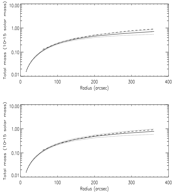
Fig. 6. The projected mass profile in the universe model: H_0 = 100 \text{ km s}^{-1} \text{ Mpc}^{-1} , \Omega_m = 0.3 , \Omega_\Lambda = 0.7 (shown as the solid line; the dotted lines mark the confidence level of 68%), and compared with that of Clowe & Schneider (shown as the dashed line). In the upper panel, the solid line presents the projected mass within 6' ; the lower panel is for the projected mass within 15' .
